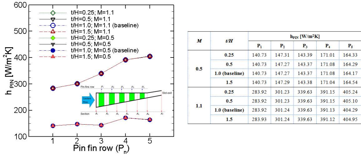
Figure 7: Comparison of heat transfer coefficient.
