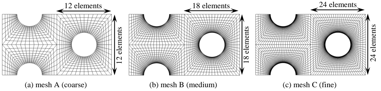
Figure 4: Three types of mesh A, B, C around the pin-fin geometry.
