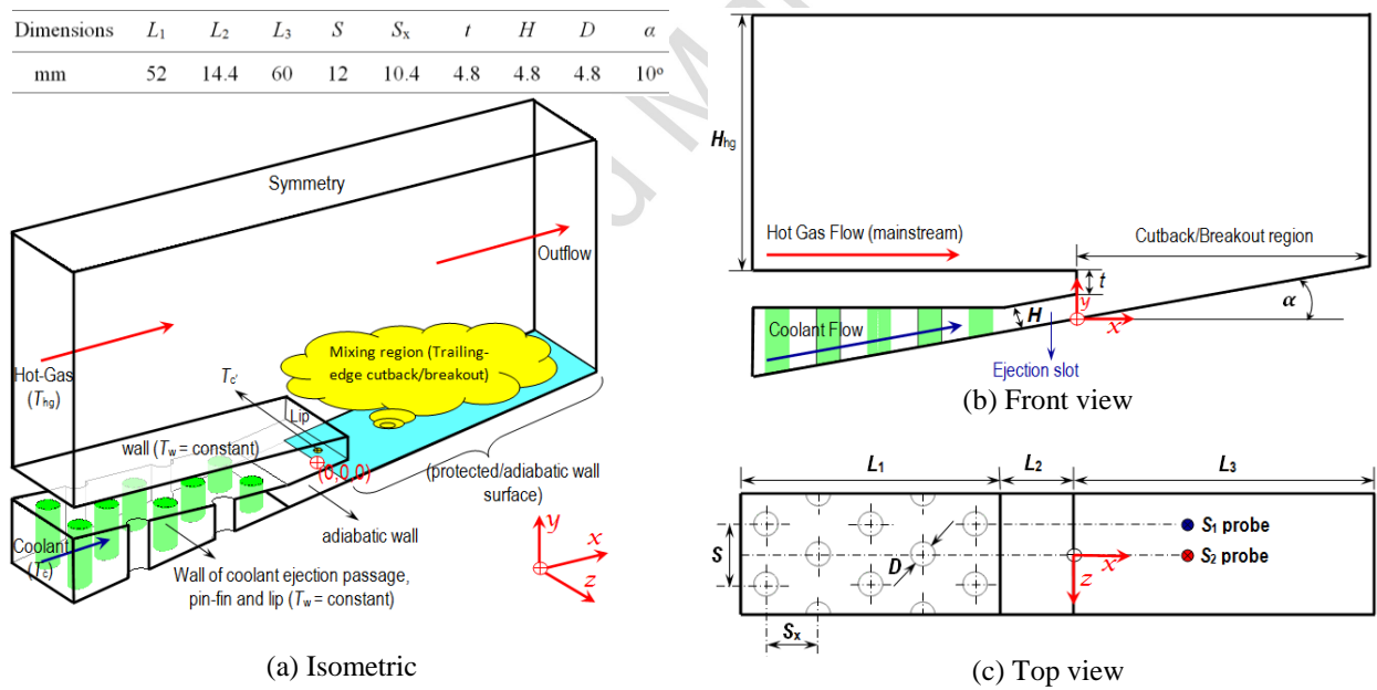
Figure 3: Computational domain, key parameters and flow conditions.
