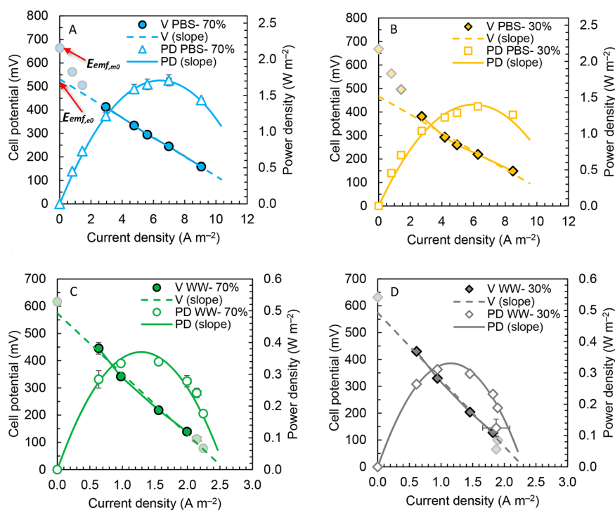
Figure 2. Modeled polarization and power density curves based on a single internal resistance calculated by the slope of the I-E_{\text{cell}} curve and several external resistances compared to the data from polarization test in (A and B) PBS and (C and D) wastewater using cathodes with diffusion layer porosities of (A and C) 70% and (B and D) 30%. The dashed lines represent the linearization of the data that would be obtained from polarization tests.
