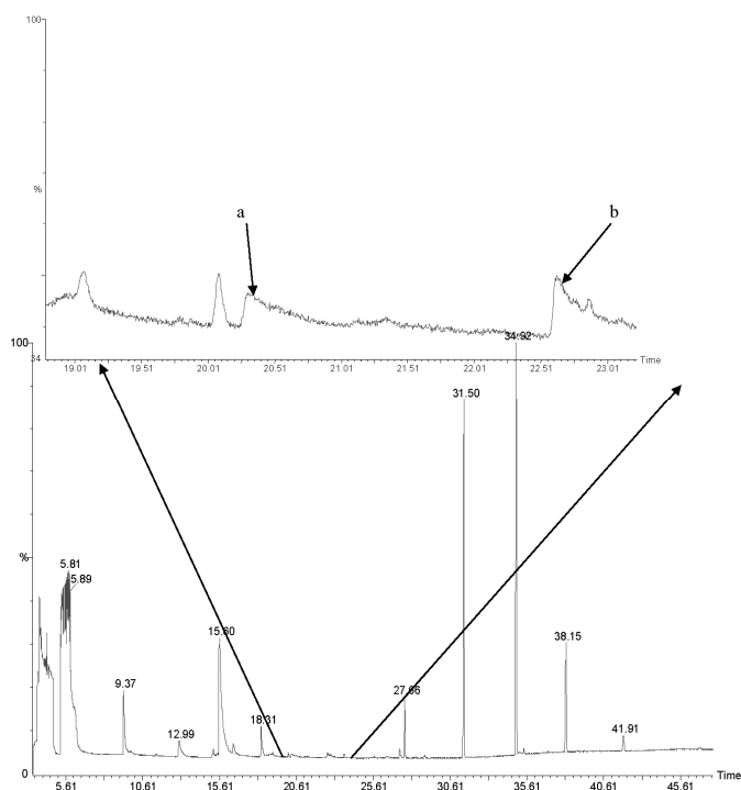
Figure 2 Typical chromatogram illustrating the VOCs extracted from the headspace above a hundred beetles of Sitophilus granarius .
