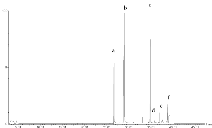
Figure 1 Typical chromatogram illustrating the major VOCs extracted from the headspace above a hundred beetles of Tribolium confusum . a = 2-methyl-1,4-benzoquinone, b = 2-ethyl-1,4-benzoquinone, c = 1-pentadecene, d = 2-methyl-1,3-benzediol, e = hexadecane and f = 4-ethyl-1,3-benzenediol.
