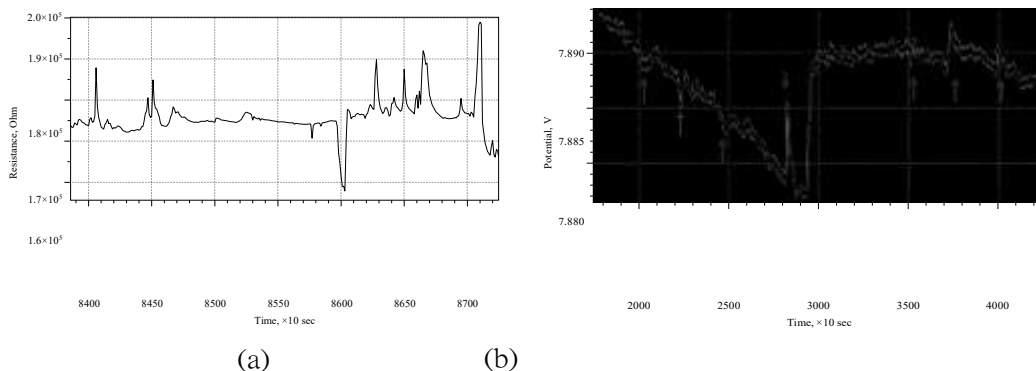
Figure 3: (a) Examples of high amplitude and high frequency spikes. (b) Oscillation of electrical potential under 10 V DC applied, where spikes analysed are marked by ‘*’. From [10].
