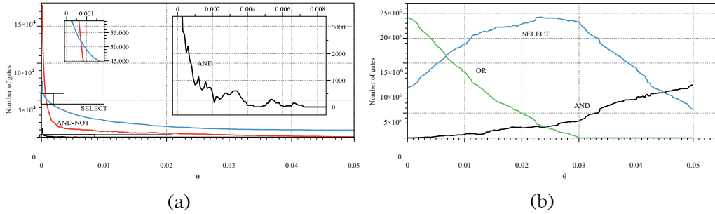
Figure 8: Occurrences of the gates from the groups and, black, or, green, and-not, red, and select, blue, for \theta [0.0001, 0.05] , with \theta increment 0.0001, in (a) fungal colony modelled with serial RC networks, (b) fungal colony modelled with parallel RC networks.
