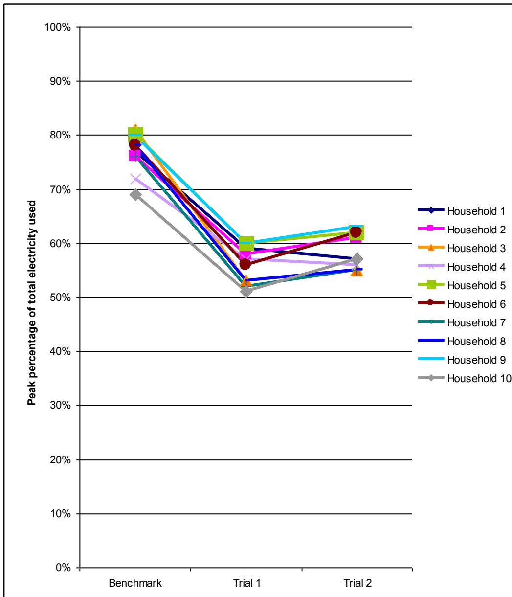
Figure 3: Comparing household peak consumption in the benchmark, Trial 1 and Trial 2 periods
