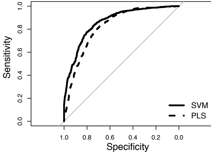
ROC curve
