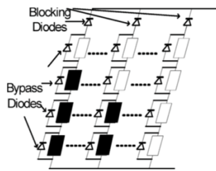
Figure 5: An example solar array with both bypass and blocking diodes present.
