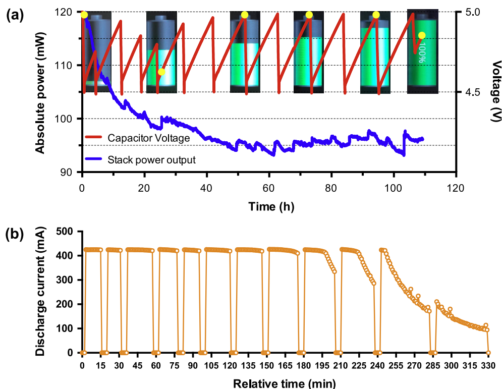
Fig. 8. Charging of the Samsung Galaxy S I9000 through its USB port (SP). (a) Power produced by the stack and voltage illustrating the charge/discharge cycles of the supercapacitor. The pictures indicate the charge state of the phone (yellow dots indicate when pictures were taken). (b) Current delivered by the supercapacitors during the discharge cycles. The time between each discharge cycle (approx. 10 h of using the phone) is not represented. (For interpretation of the references to colour in this figure legend, the reader is referred to the web version of this article.)
