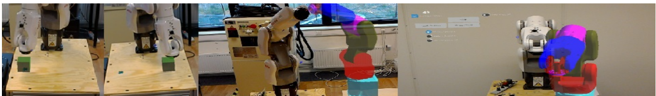
Figure 1: The view of the 3D models from the user point of view (through HoloLens). On the left, a cube that is moved by the real robot (NACHI MZ-04) through the definitions of waypoints. The 3D model of the NACHI MZ-04 that can be jogged with the user gestures (Middle). The real robot will then assume the target configuration.
