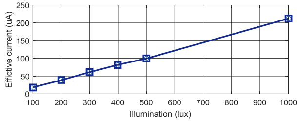
Fig. 10. Effective charge current vs. illumination condition
