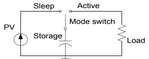
Fig. 17. Top-level circuit model of the IPEHPM with the load of an IoT node
