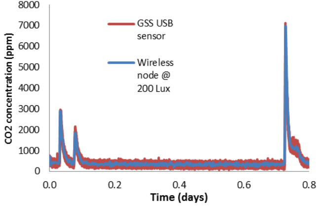
Fig. 15. Measured CO 2 concentration level traces from the IPEHPM powered IoT-based GSS sensor (blue trace) and the USB-powered one (red trace)
