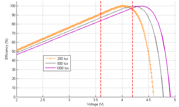
Fig. 5. Normalized output power efficiency of PV energy harvesting module vs. operating voltage at different illumination conditions
