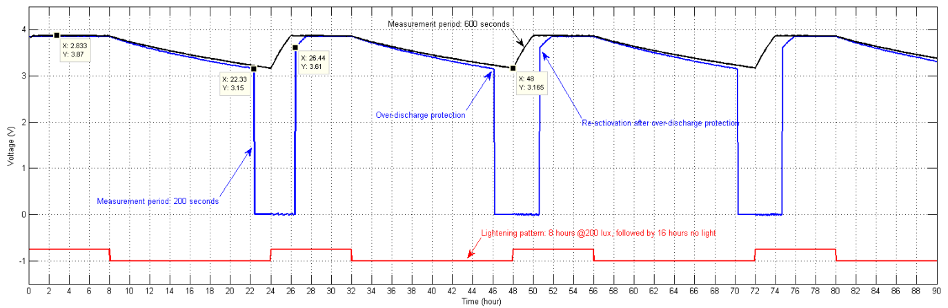
Fig. 12. Output voltage of IPEHPM measured in active mode. Blue trace is for IoT node measuring every 200 seconds and the black curve is for 600 seconds case. The daily repeated lighting pattern (red trace) is 8 hours at 200 lux, then followed by 16 hours without light. The over-discharge protection (0V output voltage of IPEHPM in active mode) and IPEHPM load reconnect (3.6V output voltage) can be observed in the blue curve
