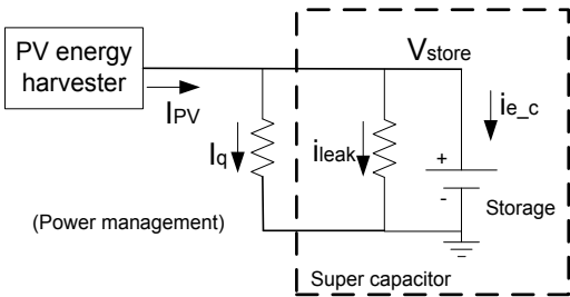
Fig. 7. Circuit diagram shown current relationship in the power module.
