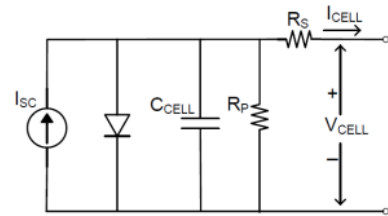
Fig. 1. Circuit model of a single PV cell which shows the PV cell as a current source and the open-circuit voltage is restricted by the diode
