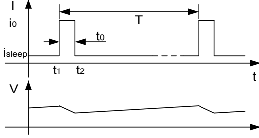
Fig. 6. Current profile and supply voltage curve when an IoT node is powered by the IPEHPM. In a measurement period of T , there is a large current pulse i_0 within t_0 (active node) and a tiny current i_{sleep} (sleep mode) during the long sleep period.
