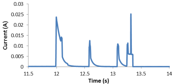
Fig. 13. Measured current profile of GSS gas sensor in low-power polling mode for one CO 2 measurement (pulses from left to right: wake-up, sensor excitation, data reading, and the data transmission)
