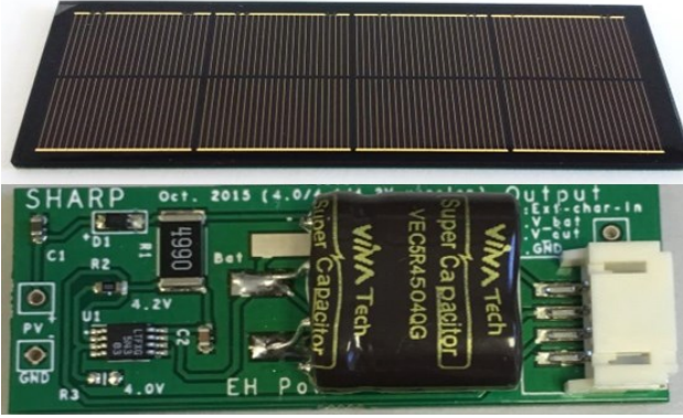
Fig. 8. The 50 mm × 20 mm × 15 mm IPENPM. Top: PV energy harvesting module side of the IPEHPM. Bottom: electronic components side of IPEHPM
