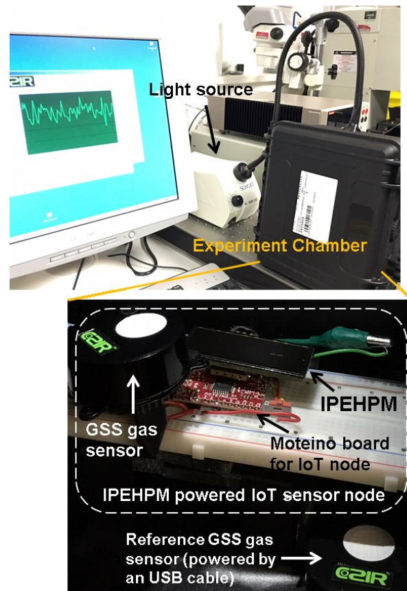
Fig. 14. Experiment set-up. Top: experiment chamber, light source and GSS GUI. Bottom: inside the experiment chamber. The dash line block shows the IoT sensor node powered by IPEHPM (GSS gas sensor, IPEHPM, and Moteino including MCU plus wireless circuits). A reference GSS gas sensor powered by an USB cable is shown in the bottom
