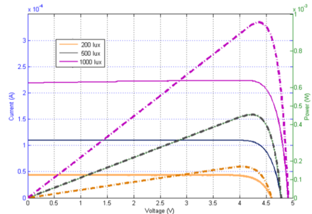
Fig. 3. I-V (solid line) and the P-V curves (dash line) of the PV energy harvesting module at different indoor illumination conditions.
