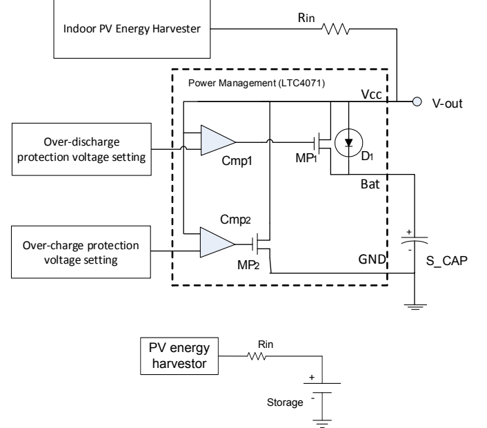
Fig. 4. Block diagram of the IPEHPM with the battery charger from Linear Technology (top) and the simplified top-level circuit of IPEHPM (bottom)
