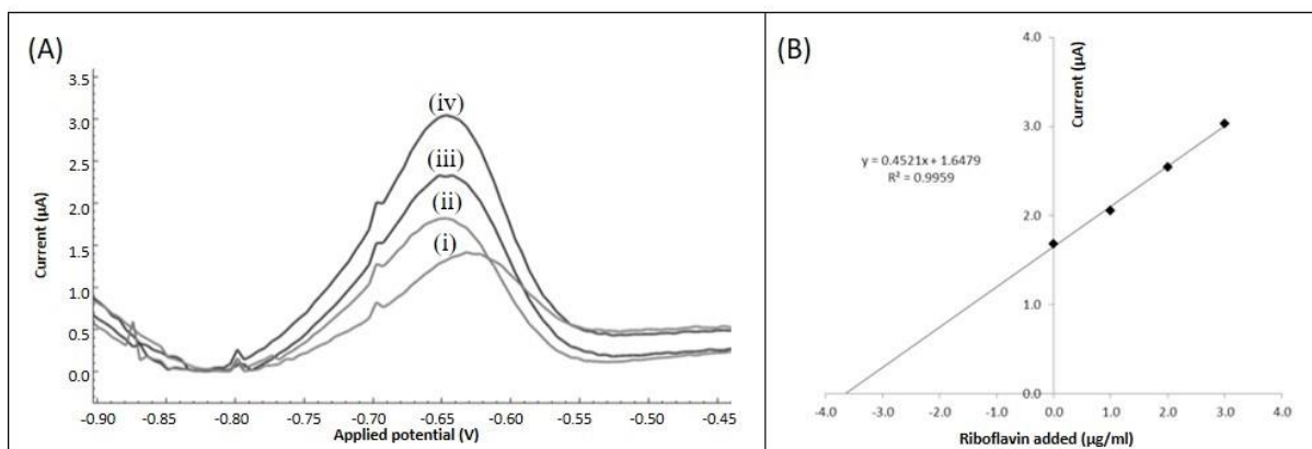
Fig. 3. (A) Square wave voltammograms were obtained using SPCEs (vs. Ag/AgCl) with a solution containing Marmite® extract in a pH 11 0.1 M phosphate buffer with 0.1 M sodium chloride with the following standard additions of riboflavin (i) 0.0, (ii) 1.0, (iii) 2.0, (iv) 3.0 µg/ml. Initial potential -1.0 V, final potential 0.0 V. Scan rate 250 mV s -1 . (B) Typical standard addition plot for riboflavin additions in a Marmite® sample using the conditions described in part A (n=5).
