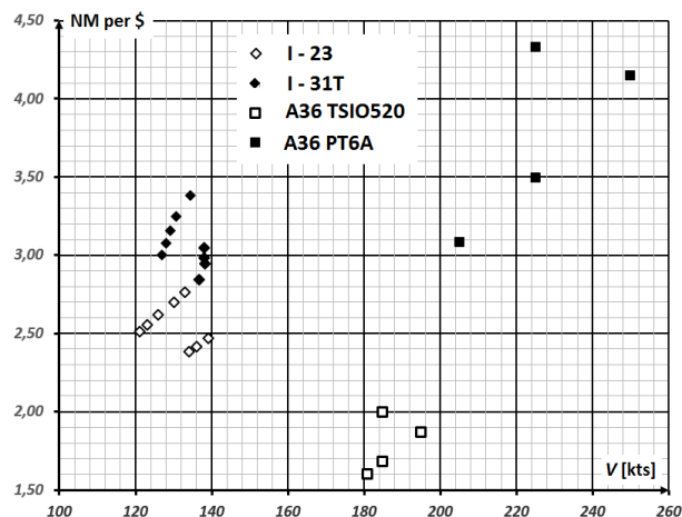
Figure 7 Distance in nautical miles flown per one US dollar by LSET aeroplane and her SEP predecessor.
