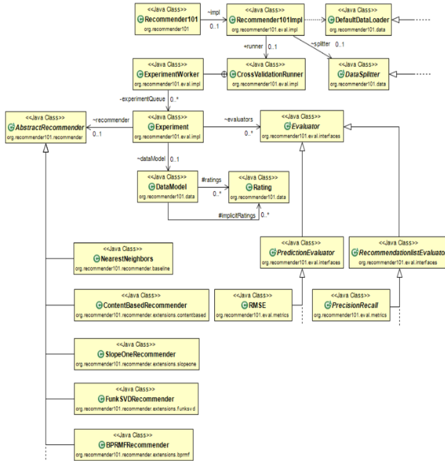
Fig 1. Recommender101 [4]
