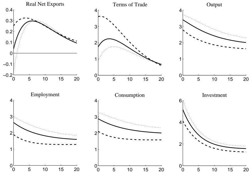
Figure 1: The Determinacy Model - Selected Home impulse responses for a 1% positive Home productivity shock: baseline (—); high trade elasticity (···); low trade elasticity (- -). Vertical axes: % deviation from the steady state; Horizontal axes: years.
