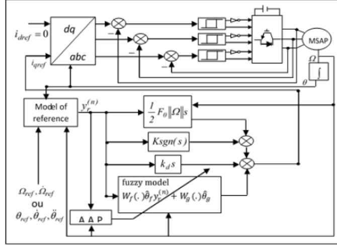
Figure 2: Speed/position control structure by the adaptive control method based on fuzzy systems.
