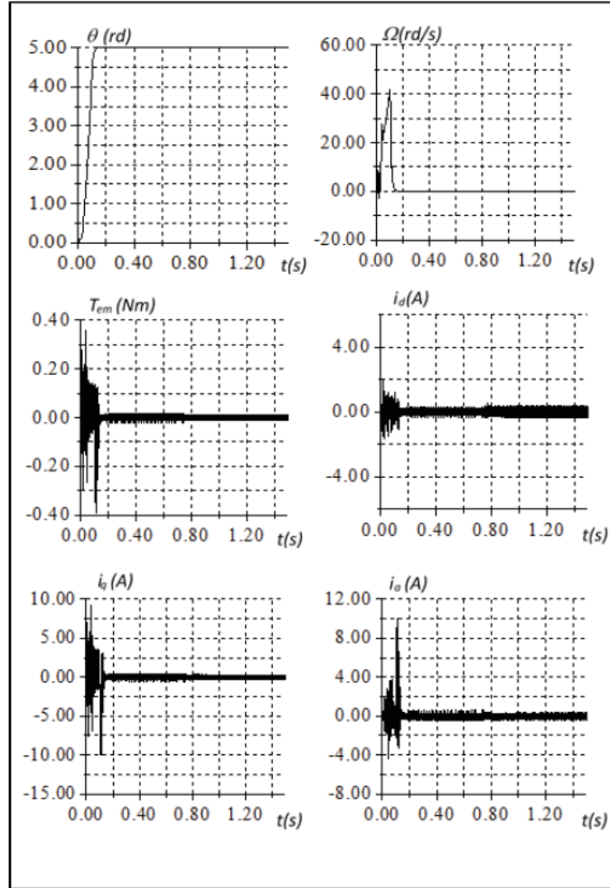
Figure 6: Dynamic behavior of the MSAP during positioning with parametric variations at time t = 0.8 s.
