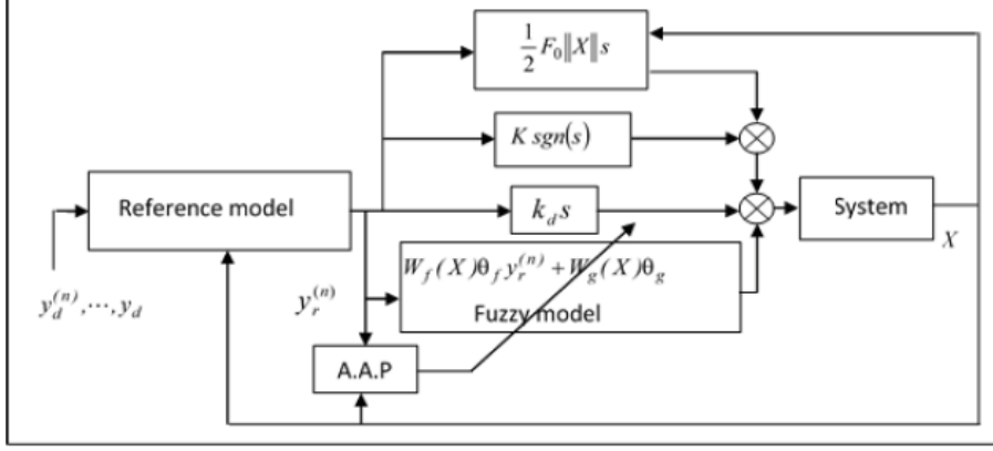
Figure 1: Structure of adaptive control based on fuzzy systems.
