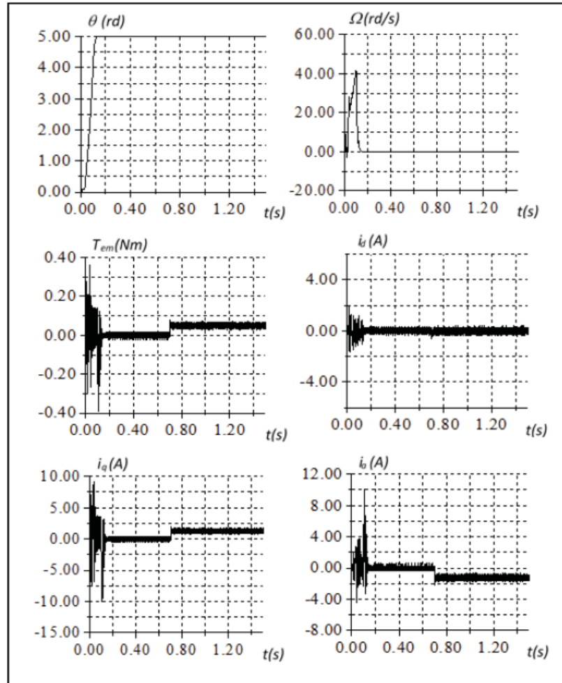
Figure 4: Dynamic behavior of the MSAP during positioning with load variation at time t = 0.7 s.
