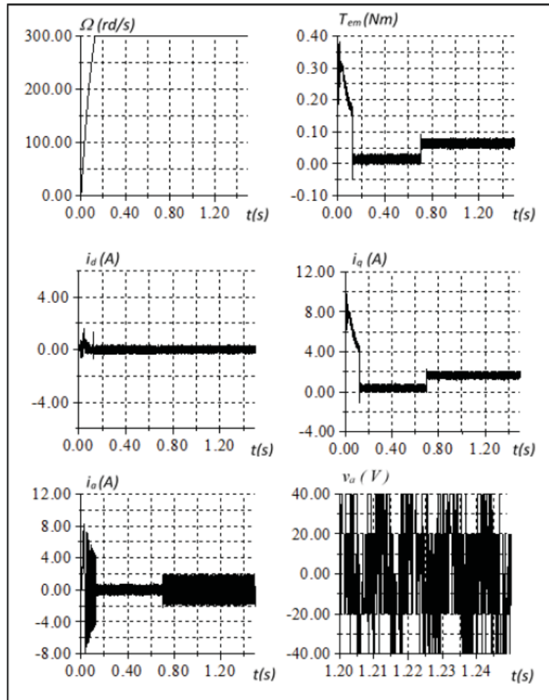
Figure 3: Dynamic behavior of the MSAP during a start-up with load variation at time t = 0.7 s.
