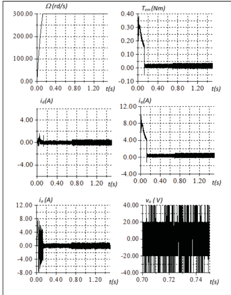
Figure 5: Dynamic behavior of the MSAP during a start-up with parametric variations at time t = 0.8 s.
