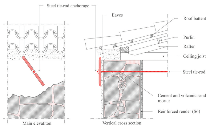
Figure 8. Improvement of the wall-to-roof connections using steel tie rods. Adapted from (Tiago Miguel Ferreira, Maio, and Vicente 2017).
