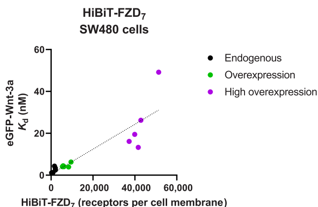
FIGURE 5 Correlation between eGFP-Wnt-3a apparent binding affinity measured with NanoBiT/BRET and number of HiBiT-FZD 7 molecules. The graphs present a correlation between eGFP-Wnt-3a K_d in nM (y-axis) and HiBiT-FZD 7 expression in molecules per cell membrane. Data points represent K_d and receptor molecule numbers come from each of n = 5 individual experiments for each condition (15 data points in total). The dotted line represents a simple linear regression fit.
