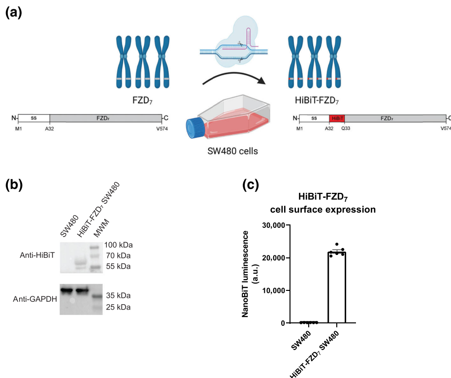
FIGURE 1 Validation of HiBiT-FZD 7 SW480 cells. (a) The scheme depicts the generation of CRISPR-Cas9 genome-edited SW480 cells expressing HiBiT-FZD 7 . ss, signal sequence (M1-A32). Generated with BioRender. (b) Validation of cellular expression of endogenous HiBiT-FZD 7 in parental and CRISPR-Cas9 genome-edited SW480 cells. Cell lysates were analysed by immunoblotting using anti-HiBiT antibody and anti-GAPDH served as a loading control. The predicted molecular weight of HiBiT-FZD 7 = 62.0 kDa. Western blot experiments were repeated five times with similar results. MWM, molecular weight marker. (c) Surface expression of HiBiT-FZD 7 was quantified by measuring NanoBiT-emitted luminescence. Raw data are shown from n = 6 individual experiments and are presented as mean \pm SEM.
