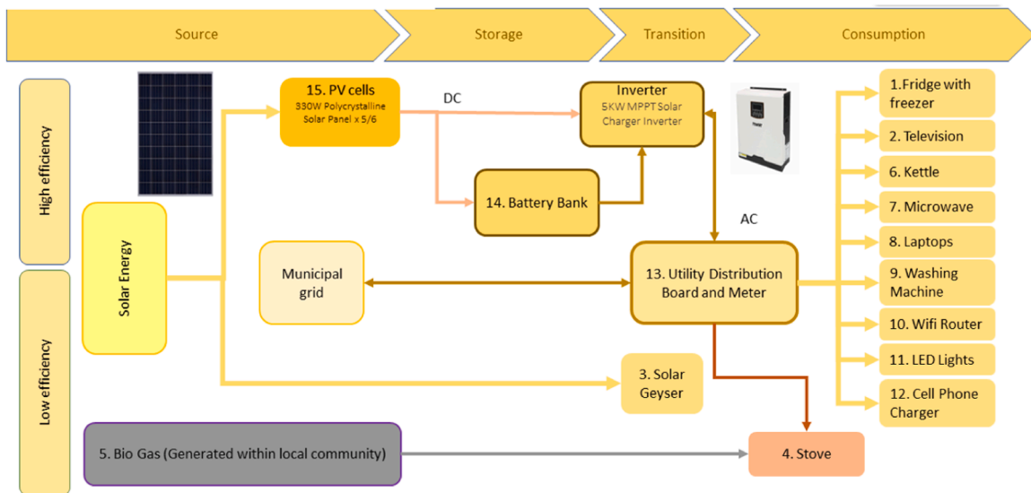
Fig. 7. Energy and water usage design concepts. Source Phiri and Bosa. 2021.
