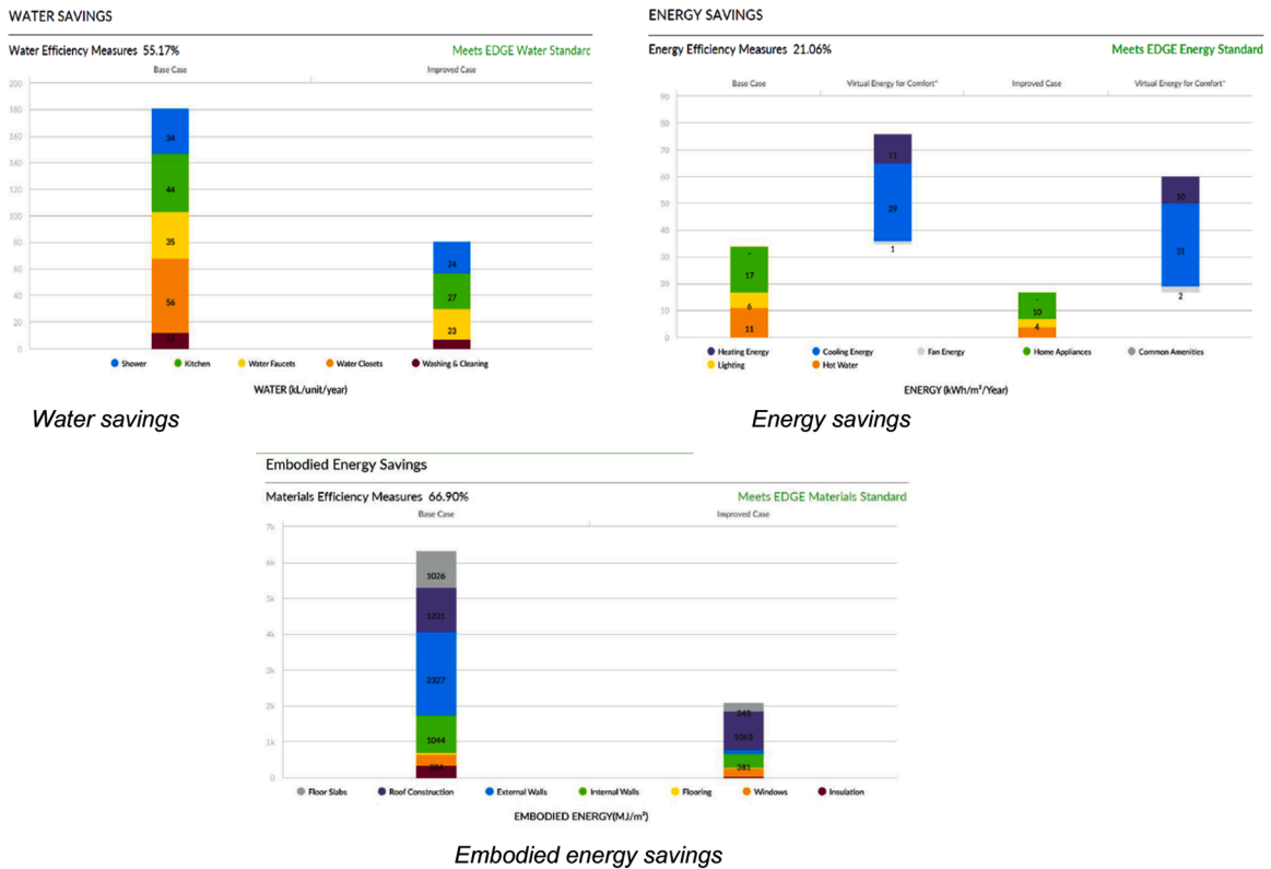
Fig. 8. Building performance of SIAH-Livable.
