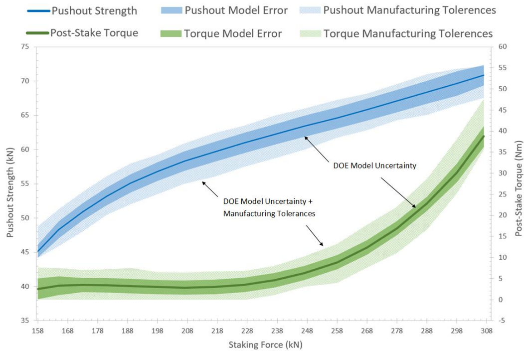
Figure 5. Example of the staking design tool output. The Inner and outer shaded bands represent a 95% confidence interval for the model's inherent uncertainty and the combination of the model's uncertainty and manufacturing tolerances, respectively.
