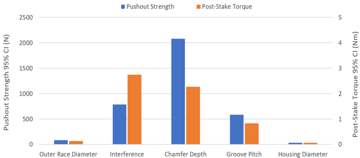
Figure 6. Impact of manufacturing tolerances
