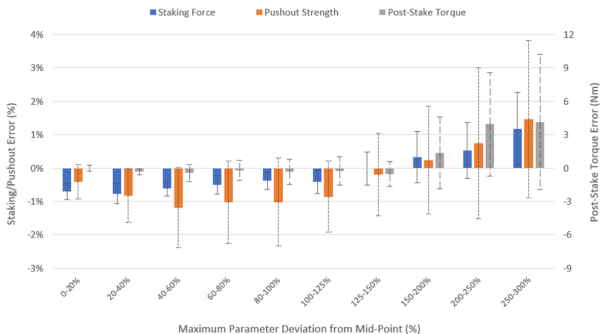
Figure 4. DOE model error with 95% confidence intervals.
