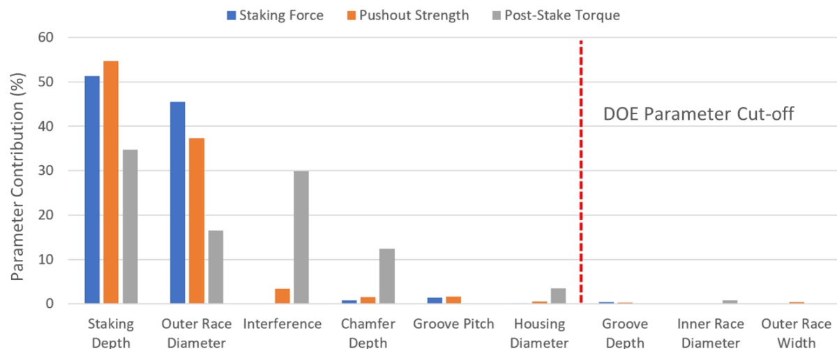
Figure 2. Relative contribution for each DSD parameter
