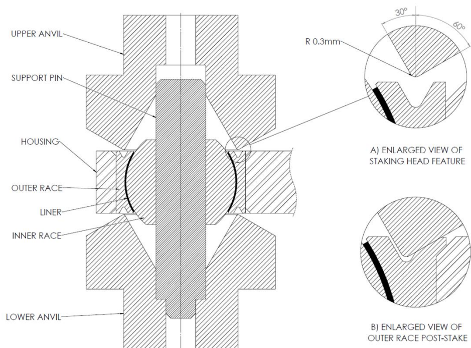
Figure 1. Cross-sectional schematic of the staking process
