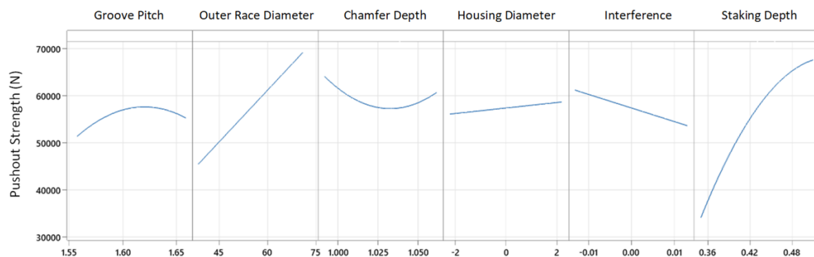
Figure 3. The main effects plot for pushout strength; showing a non-linear response for groove pitch, chamfer depth and staking depth. All dimensions in mm
