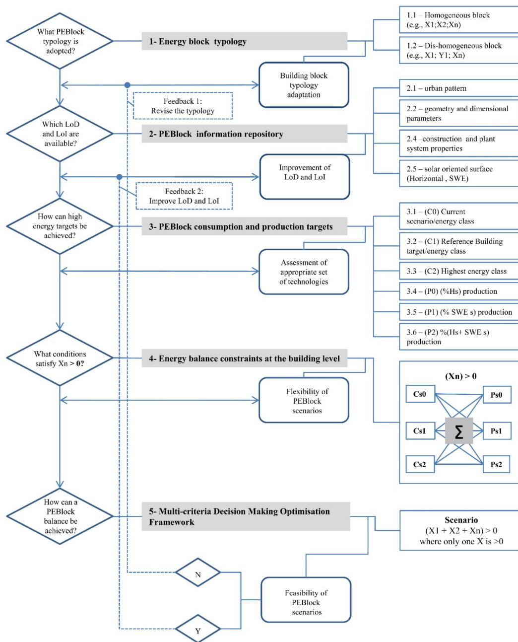
Figure 1. Workflow structure.
