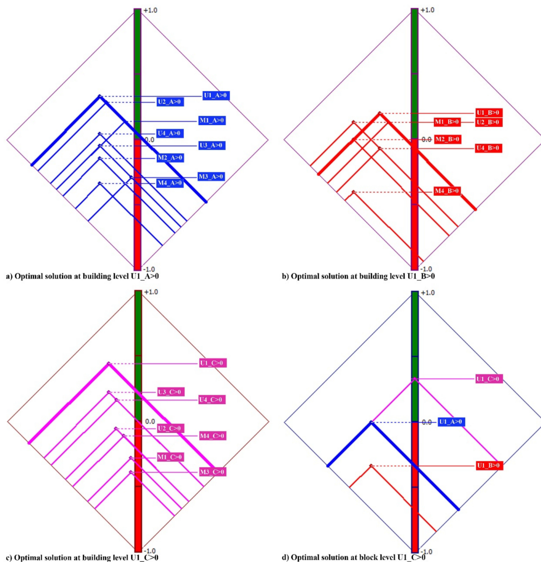
Figure 6. Actions comparison.
