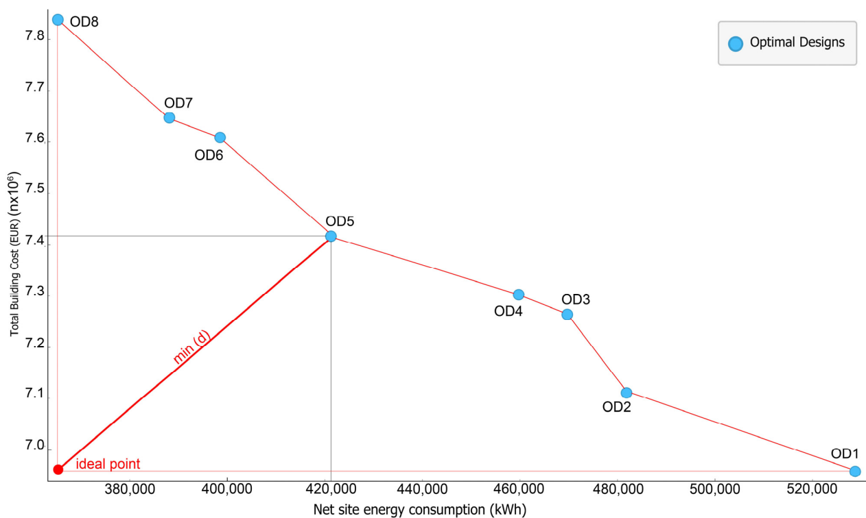
Figure 4. Optimal design solutions without PV integration.
