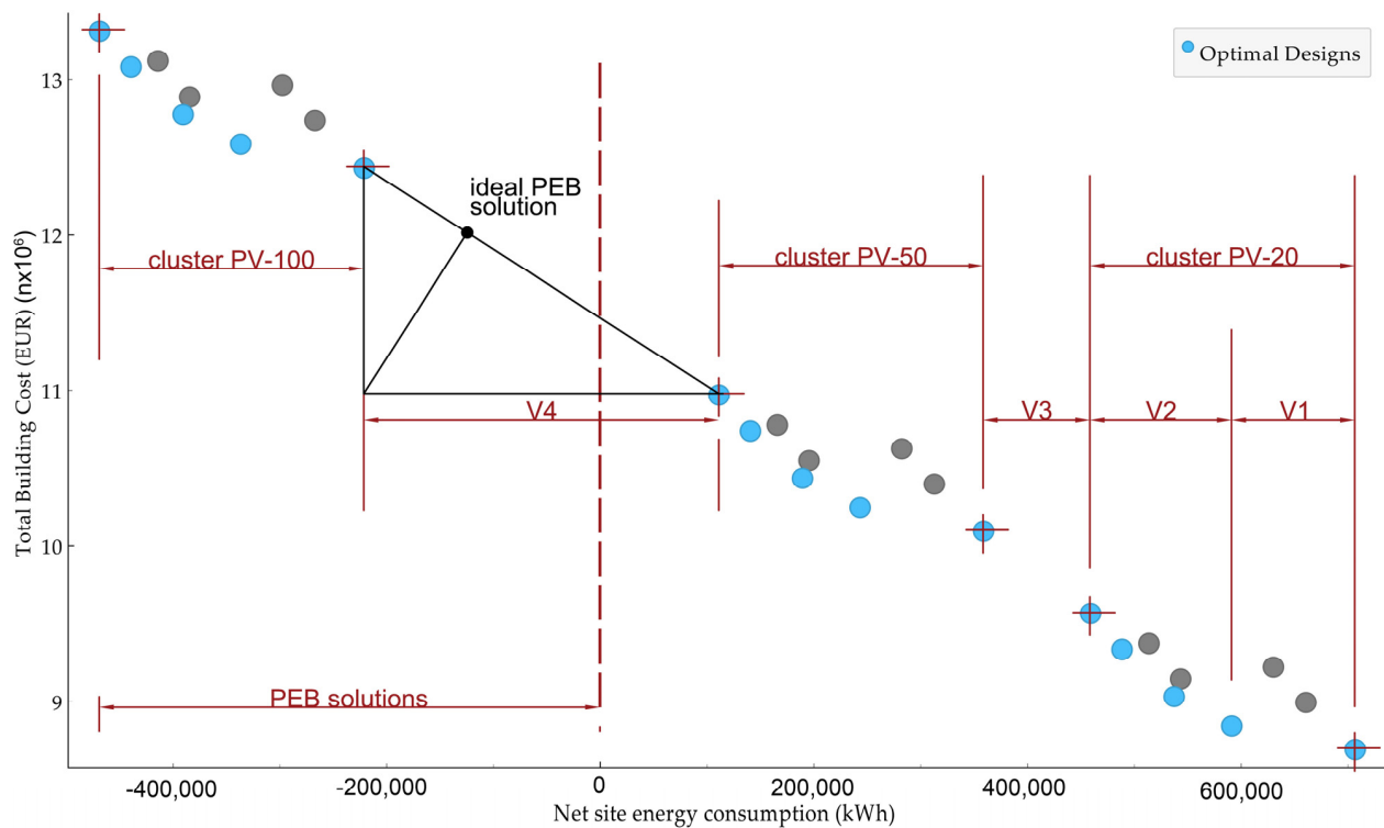
Figure 7. Pareto front: design solutions with PV integration.
