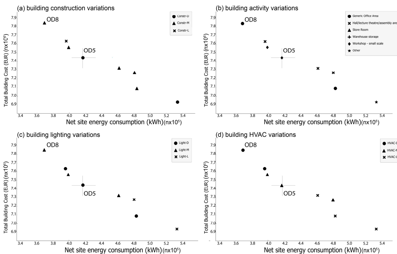
Figure 5. Main variables related to the optimal design solution. (a) Building construction variations; (b) Building activity variations; (c) Building lighting variations; (d) Building HVAC variations.
