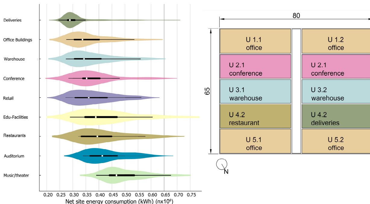
Figure 6. Building activity variations related to the net site energy consumption.
