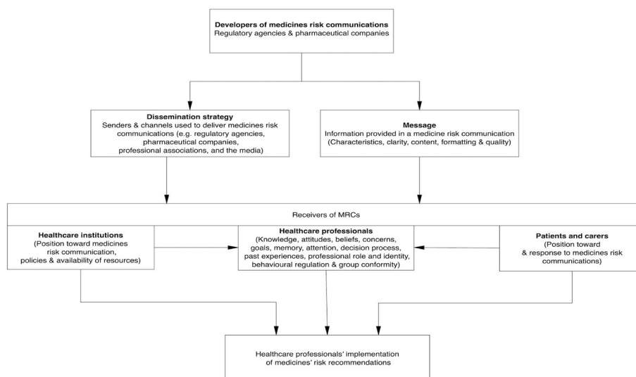
Fig. 3. Concept mapping.
