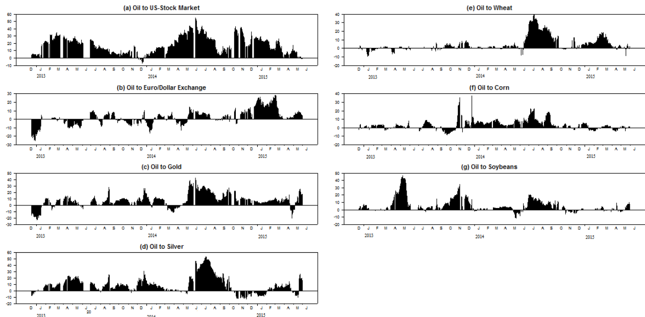
Figure 5: Pairwise directional net volatility spillovers between the crude oil market and other markets
