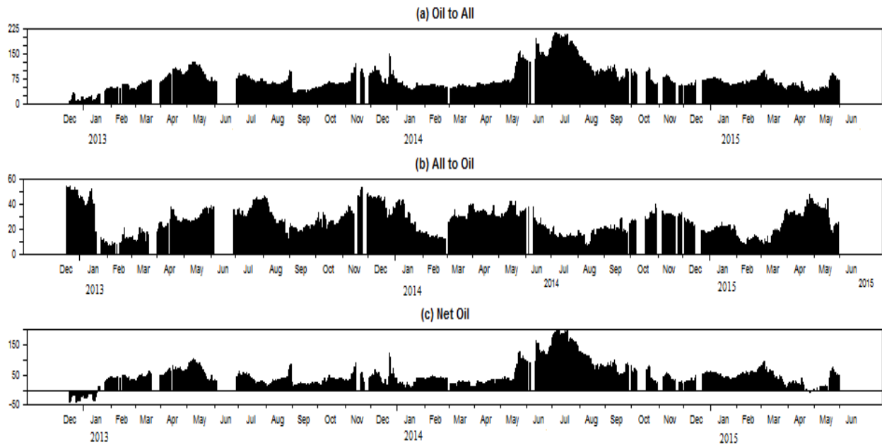
Figure 4: Direction of implied volatility spillovers
