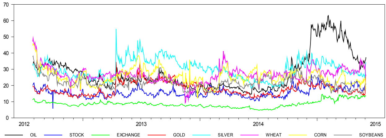
Figure 1 A: Time series plot of the implied volatility index in level
