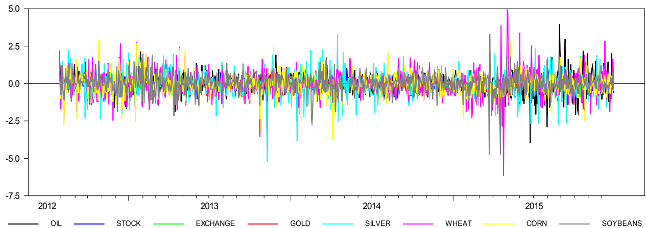
Figure 1B : Time series plot of the implied volatility index in log changes
