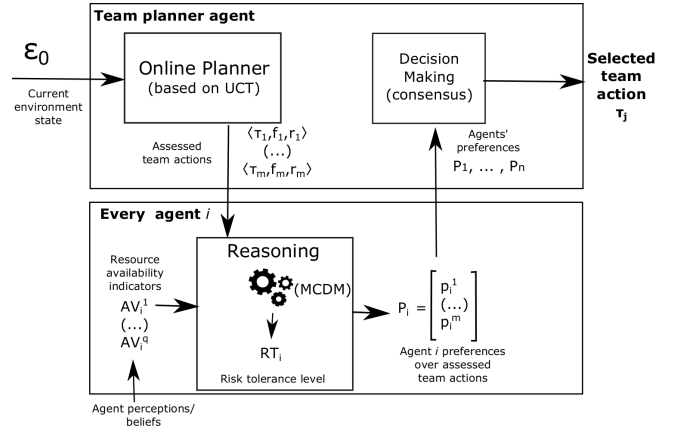
Fig. 2. Architecture of the risk-aware multi-agent planning framework
