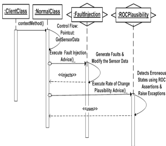
Figure 4 Rate of Change Aspect Pattern Dynamics
