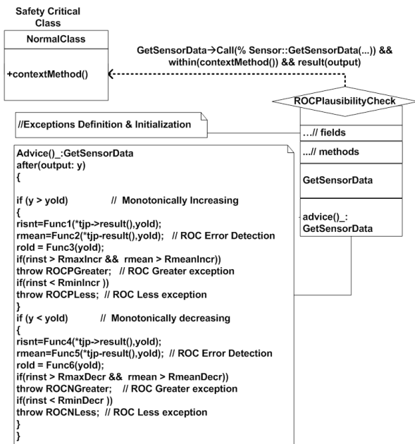
Figure 3 Rate of Change Aspect Pattern Structure
