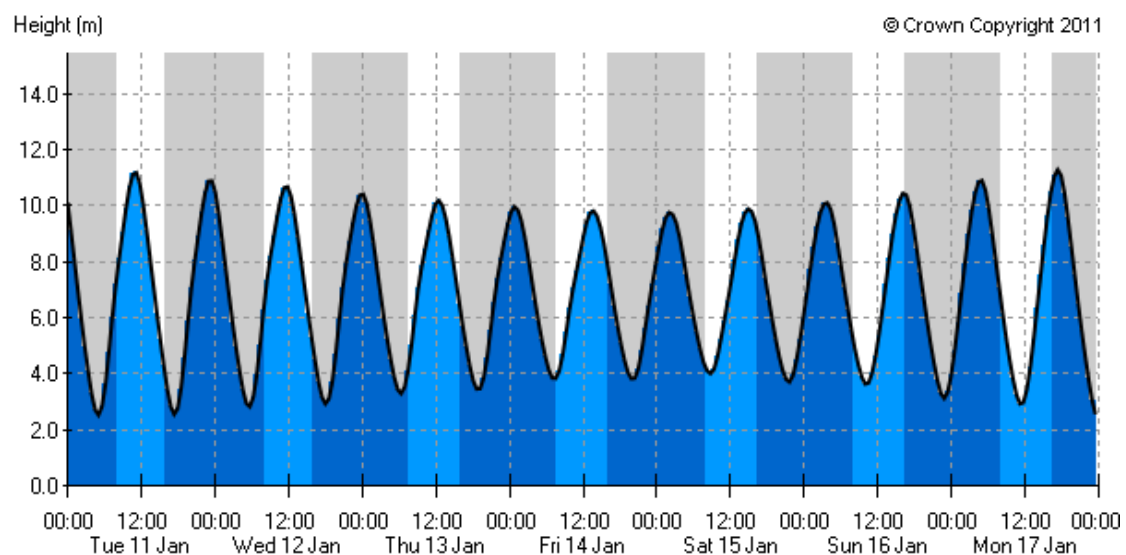
Figure 1. A week's tide timetable for Port of Bristol (Jan 2011) Crown Copyright.
