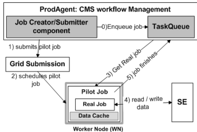
Figure 4: Overview of the proposed architecture
