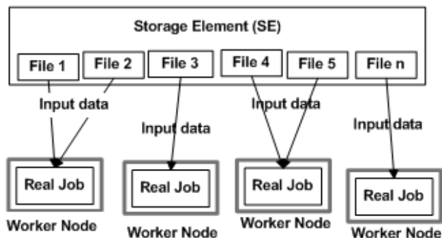
Figure 2: Multiple jobs accessing an SE
