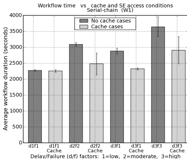
Figure 9: Workflow turnaround time under different SE conditions
