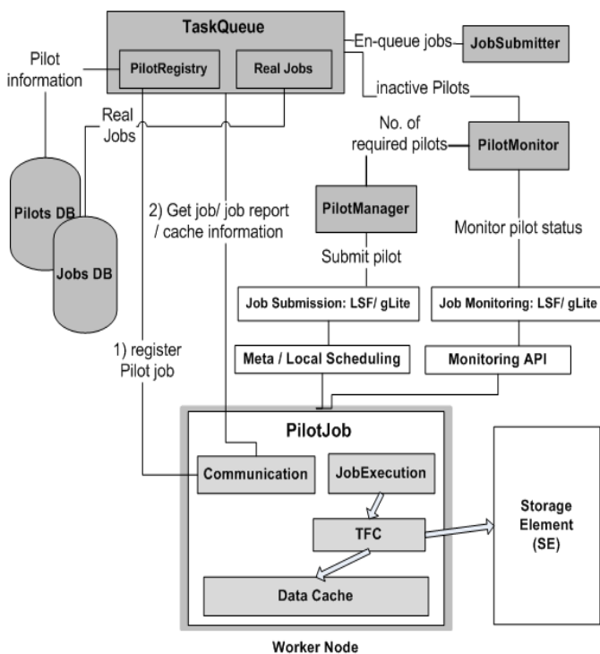
Figure 5: Detailed architecture of PilotJob and TaskQueue
