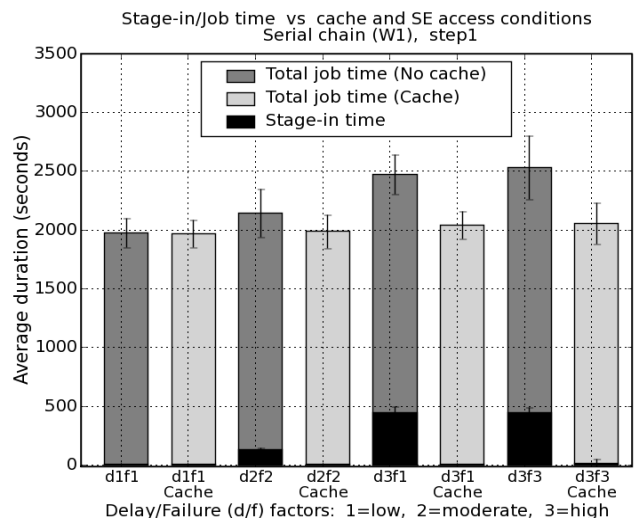
Figure 8: Effect of data cache on stage-in time under different SE conditions
