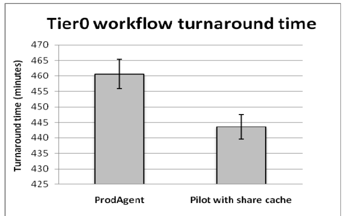
Figure 6: Effect of pilot-based system on the Tier0 workflow turnaround time
