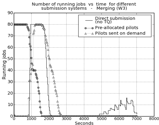
Figure 7: Number of running jobs over time
