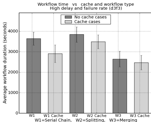
Figure 11: Workflow turnaround times for different workflow types
