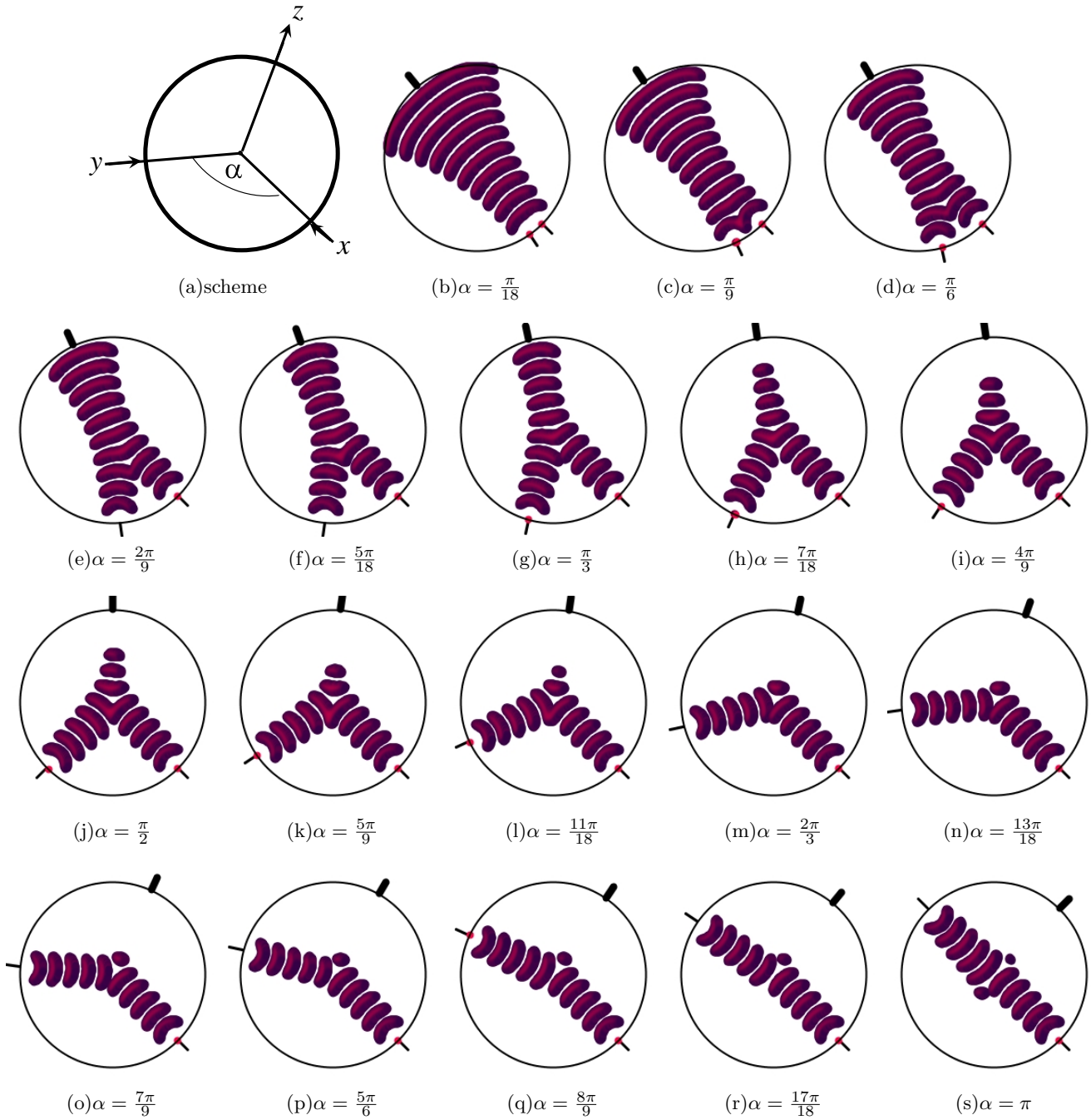
Fig. 2. Outcomes of collisions between two wave-fragments x and y approaching each other at angle \alpha , illumination level is \phi = 0.07873 ; z shows orientation of z velocity vector of the resultant wave-fragment, produced in the collision.
