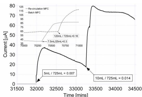
Fig. 4 Response curves from re-circulating and batch mode MFC. The main graph shows the fast response from direct injections in re-circulation mode, at carbon-energy limited concentrations. The inset shows the response curves from the same re-circulation mode MFC as well as from a batch mode MFC, when fed with high doses of urine.
