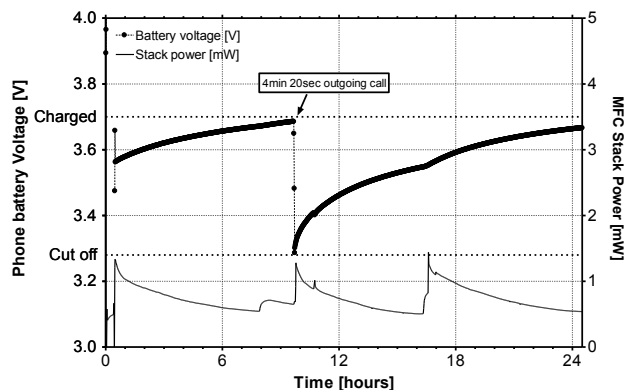
Fig. 6 MFC stack (24x 6.25mL units) powering the Samsung mobile phone, when fed with neat urine.
