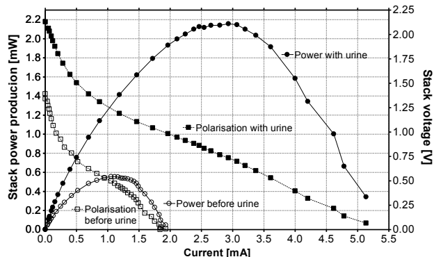
Fig. 3 Power and polarisation curves from the ceramic 12x MFC stack, when fed with acetate/tryptone-extract (open symbols) and urine (closed symbols).
