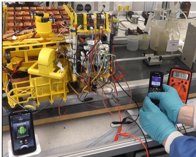
Fig. 7 Snapshot of the outgoing voice call made by the MFC powered Samsung E2121 (right) to the receiving HTC mobile handset (left); the digital multi-metre on the far right, shows the battery voltage.
