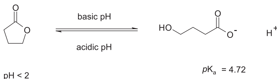
SCHEME 1 Solution pH behaviour of GHB and GBL
