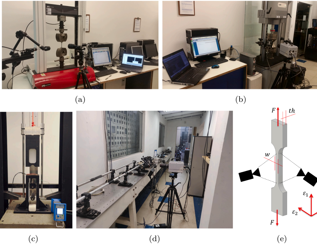
Fig. 4. Equipment used for performing mechanical characterization tests under a wide range of strain rates (a) Instron 3369, (b) Instron EletroPuls E10000, (c) Testing rig that uses the energy of falling mass for performing a tensile test, (d) Split Pressure Hopkinson Bar and (e) specimen local reference used.
