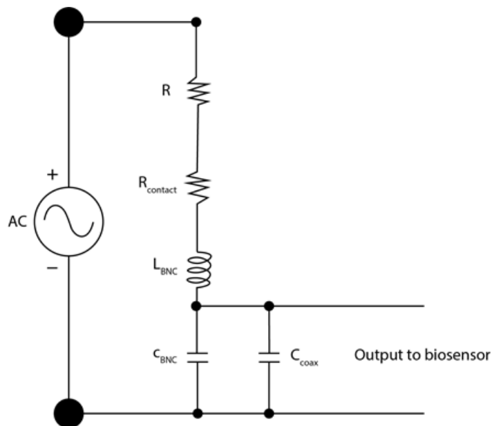
Fig. 4a) EEC for the ZnO nanoparticle biosensor modelling the constituent layers of the biosensor: PCB electrode, PET-ZnO substrate, antibody functionalised ZnO in contact with PBS, bound CRP antigen and finally the bulk PBS buffer solution and fig 4b) Electrical circuit model representing the C60 instrument front-end impedance components and coax cable connection to the biosensor.
