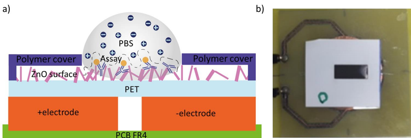
Fig. 1. a) Schematic representation of the NFIS ZnO biosensor structure and b) top-view image of The PET-ZnO biosensor chip positioned on the co-planar sensing electrode.
