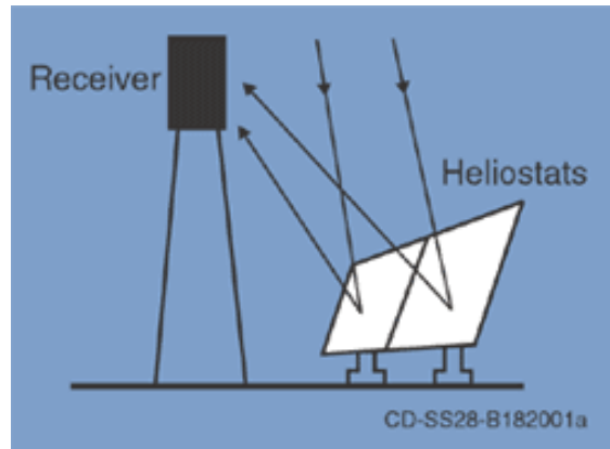
Figure 6: Power Tower System for Concentrating Solar Power.
