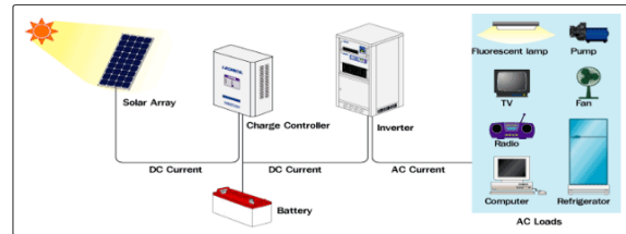
Figure 4: Diagram of a rooftop based solar panel system.
