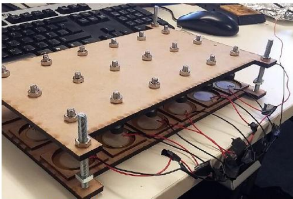
Figure-8. Prototype Harvester with piezo sensors
