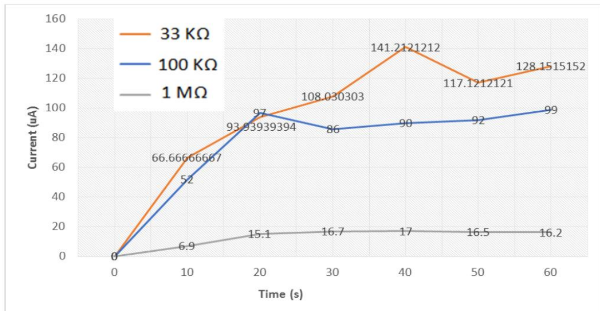
Figure-14. Depicts current output with various loads
