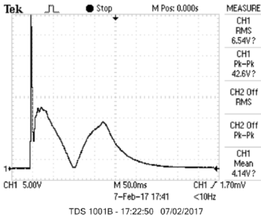
Figure-6. Individual piezo rectified
