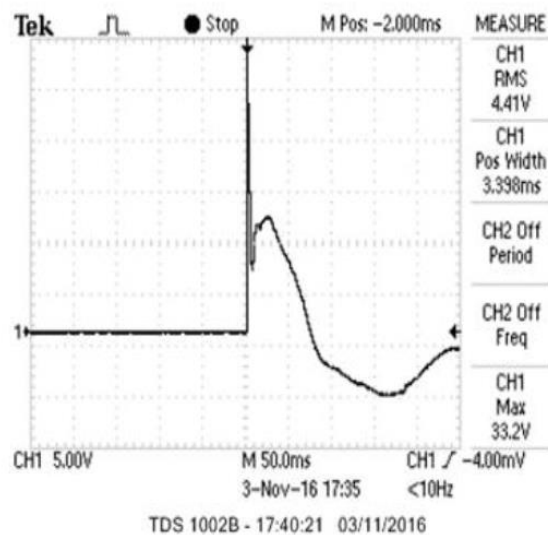
Figure-4. 4-5 rms volts output from piezo disc
