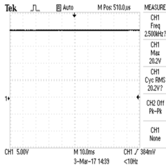
Figure-11. Shows after 60 seconds of stepping 20.2Volts is generated
