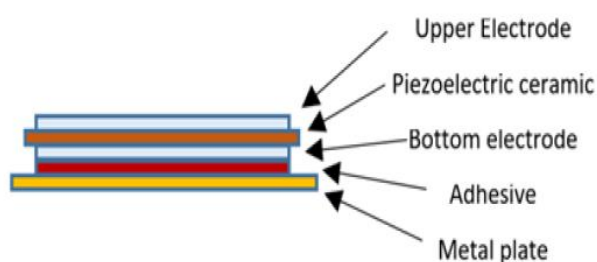
Figure-3. Structure of piezo disc
