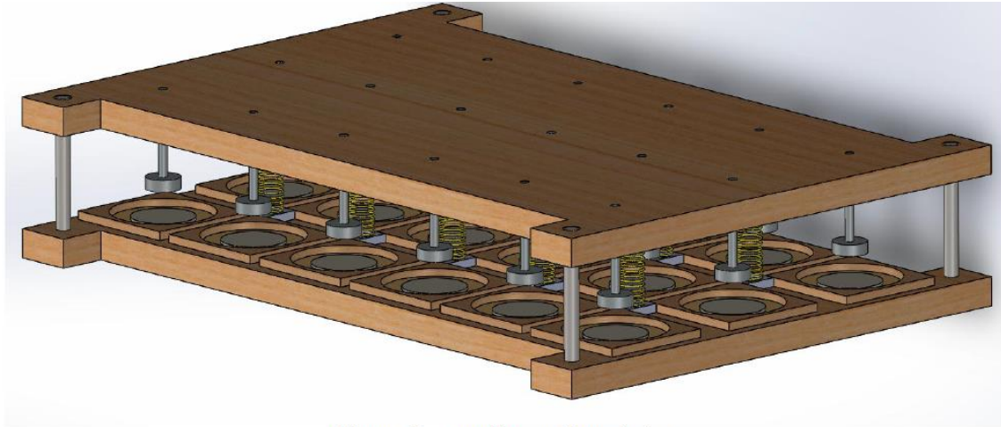
Figure-7. Prototype Harvester isometric view
