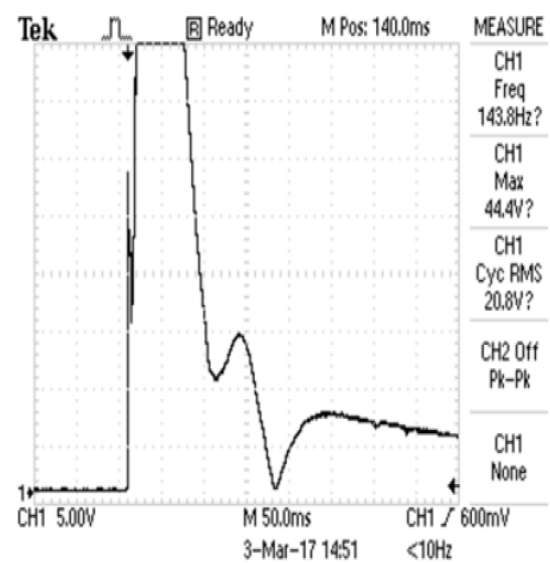
Figure-12. Depicts the Output voltage from one step
