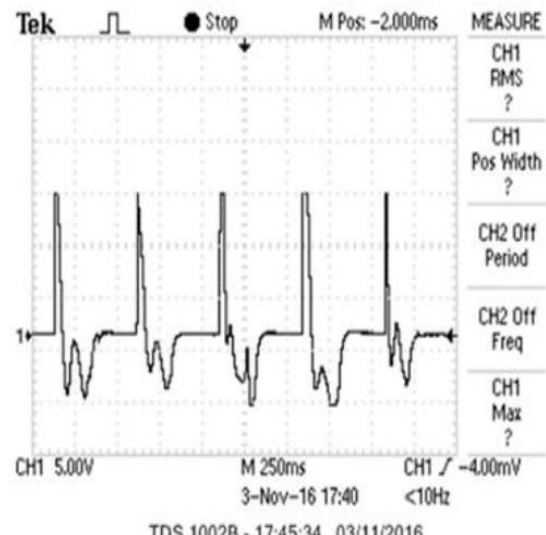
Figure-5. Piezo output from firm tapping
