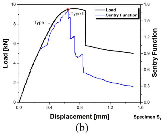
Fig. 11. The sentry function curves of specimens a) S_{M-K} and b) S_4 .
