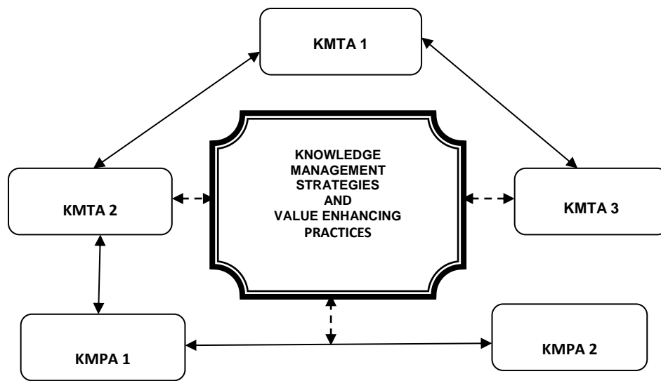
Figure 2: Framework components
