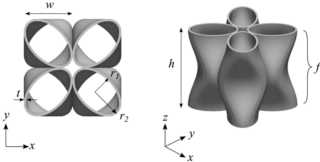
Fig. 1. Annotated circular honeycomb (2x2) with geometric parameters of the unit cell.
