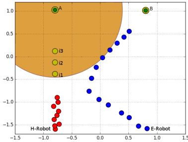
Figure 7: The tested behavioural alternatives for the initial plan (yellow dots), are the A and B objects, and the intercept points i1-i3. The E-robot path (blue dots) moves to intercept the H-robot (path in red dots). The H-robot stops when the E-robot approaches within 0.5m. The E-robot then continues to the safe object B, and stops 0.5m from it (due to collision avoidance). The orange circle shows the E-robot and H-robot danger thresholds.
