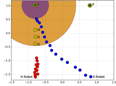
Figure 8: The tested behavioural alternatives for the initial plan (yellow dots), are the A and B objects, and the intercept points i1-i3. The E-robot path (blue dots) moves to intercept the H-robot (path in red dots). The H-robot stops when the E-robot approaches within 0.5m. The E-robot then continues to object A as it was commanded by the H-robot, and stops 0.5m from it (due to collision avoidance). The orange circle shows the E-robot and H-robot danger thresholds. The purple circle is the robot objective distance threshold.
