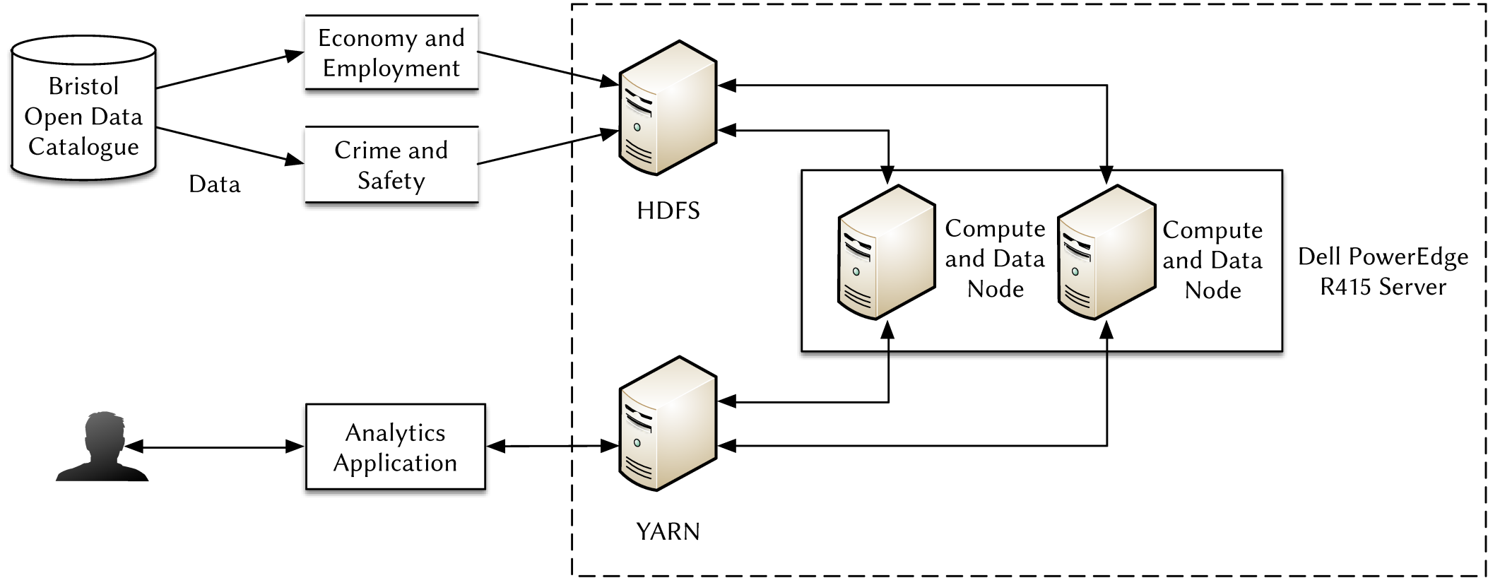
Hadoop-based Cloud Infrastructure-as-a-Service
