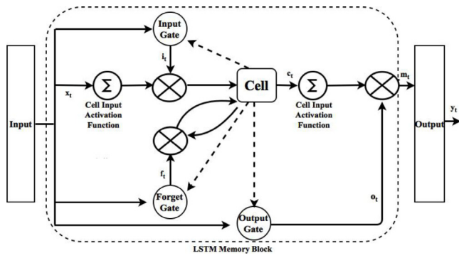
Fig. 1. LSTM block diagram (Singh, Chauhan, Krishnamachari, & Vig, 2015).
