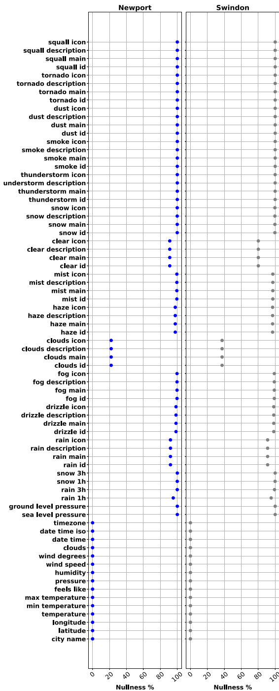
Fig. 15. Nullness of features in the cities of Newport and Swindon.
