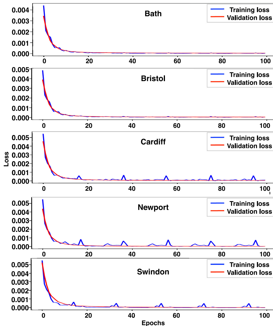
Fig. 10. Training and validation loss - Model 4.
