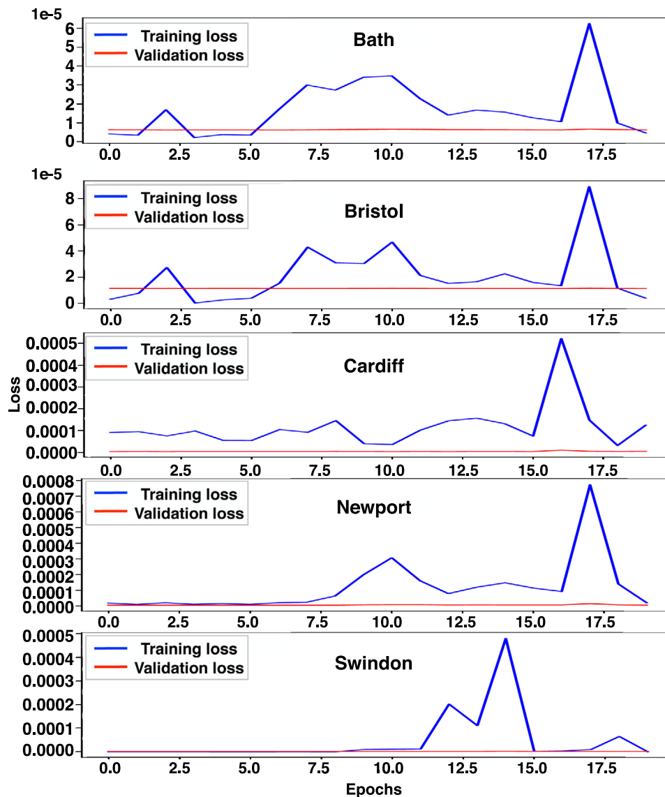
Fig. 7. Training and validation loss - Model 1.
