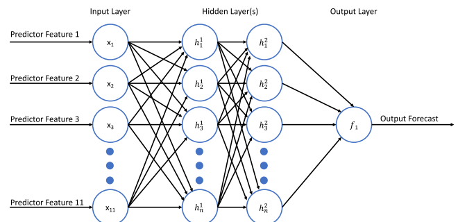
Fig. 6. General Neural Network architecture.
