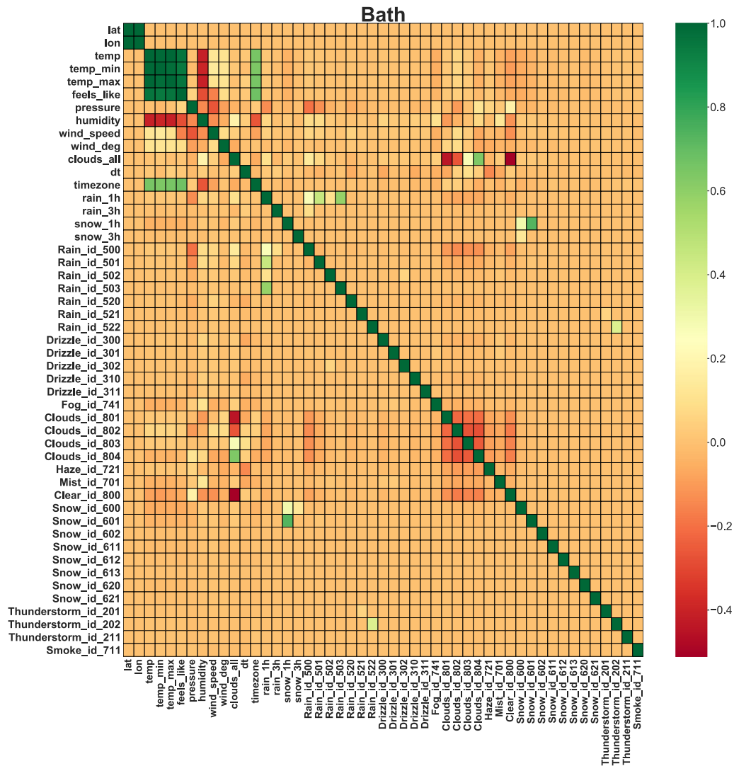
Fig. 3. Correlation Matrix of the city of Bath.
