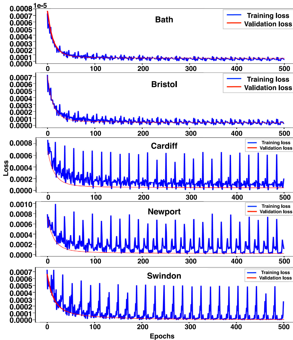
Fig. 8. Training and validation loss - Model 2.
