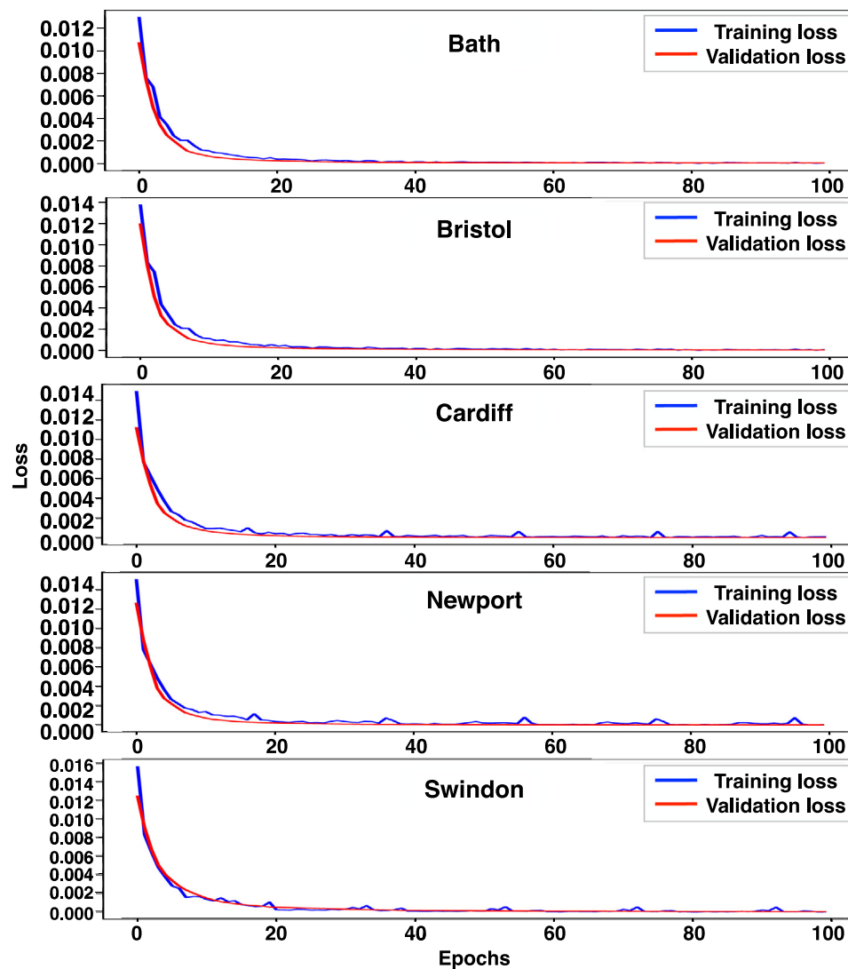
Fig. 9. Training and validation loss - Model 3.
