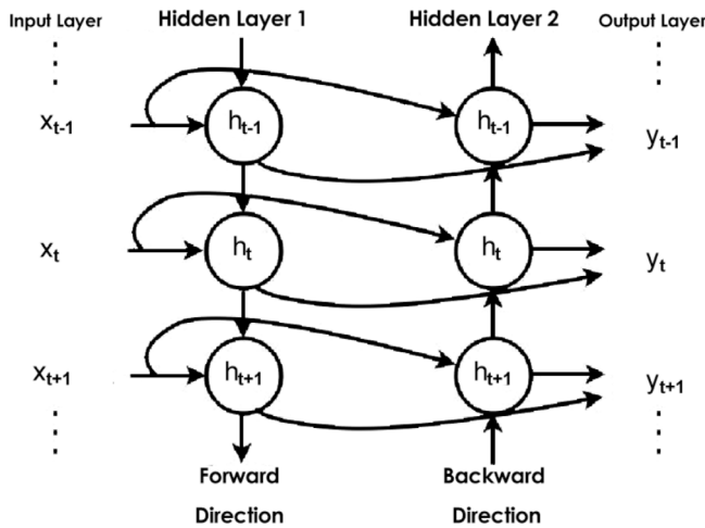
Fig. 2. Bidirectional-LSTM Network architecture (Singh et al., 2015).
