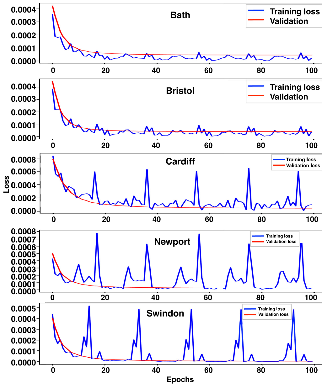
Fig. 11. Training and validation loss - Model 5.
