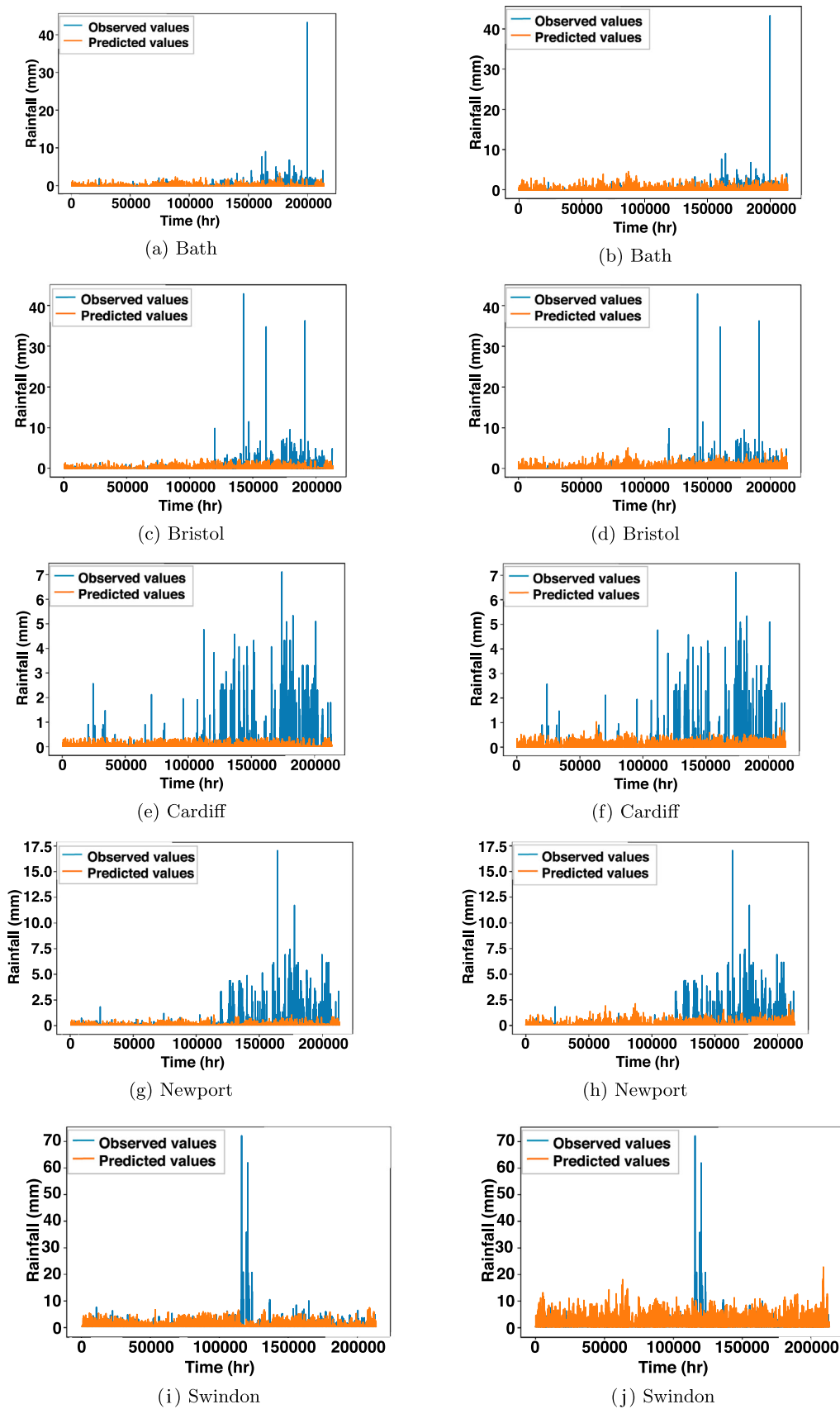
Fig. 16. Observed rainfall vs. Predicted rainfall (left: Model 4, right: Model 6).
