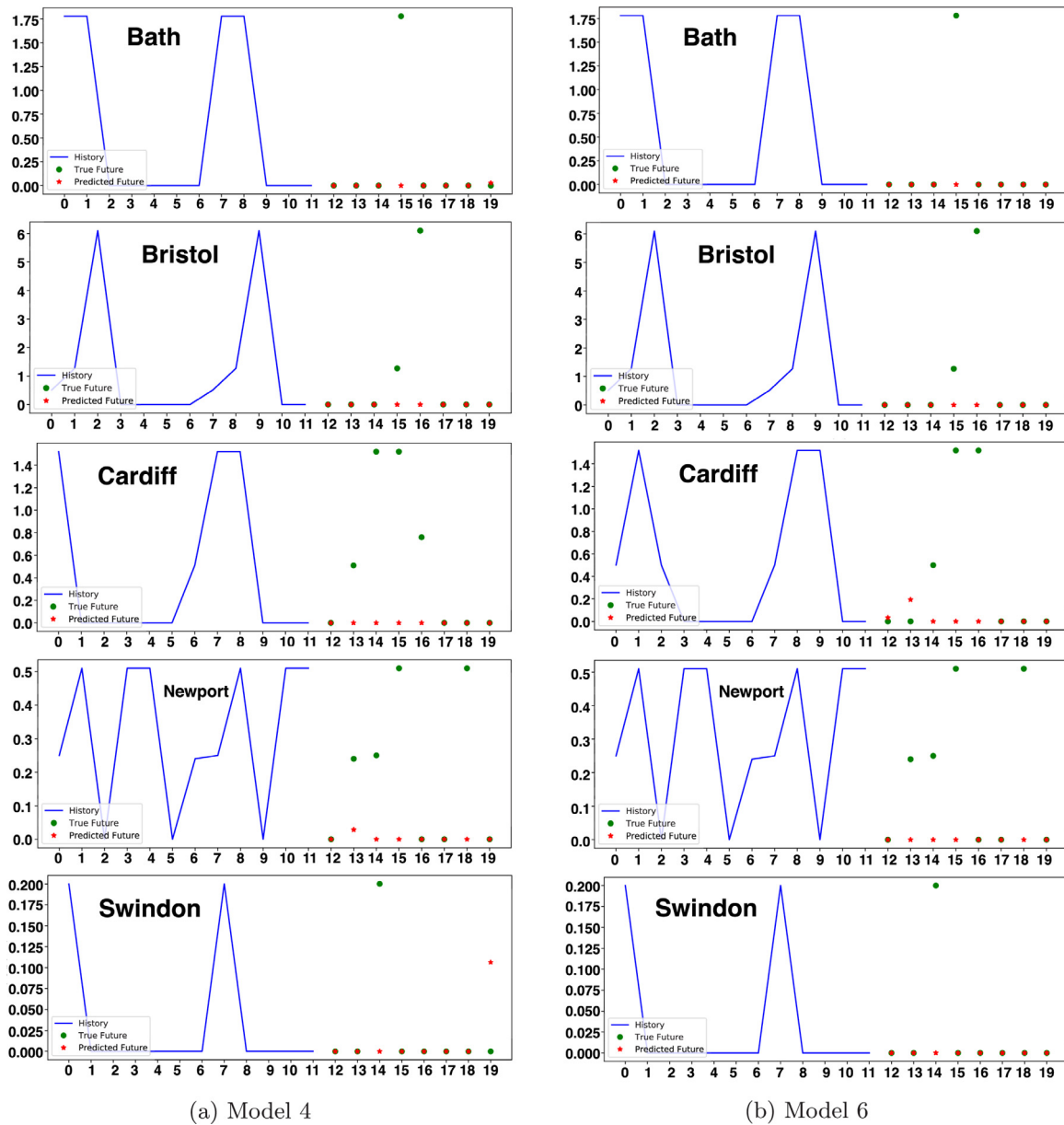
Fig. 13. Examples of rainfall predictions and true observed rainfall.
