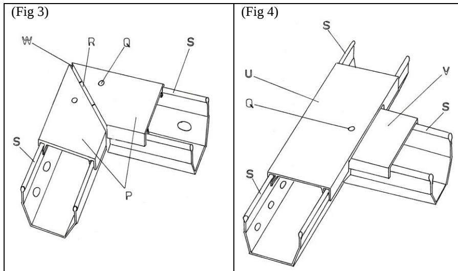
Figures 3 and 4: Sectional drawing to illustrate the new pivotally connected elbow-bend with internal deflector and the pivotally connected T-piece with internal deflector plate.
