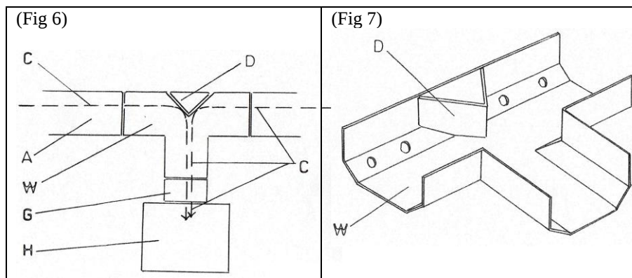
Figure 6 and 7: Plan drawing to illustrate water and/or sediment flowing into the sump/pump chamber. Plus a sectional drawing of the new T-piece to show the internal water deflector plate that also acts as a support for the T-piece soffit
