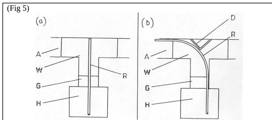
Figure 5: Plan views of the perimeter floor drain, T-piece, link drain and sump chamber to show the accessibility provided by the new pivotally connected T-piece with water deflector plate.
