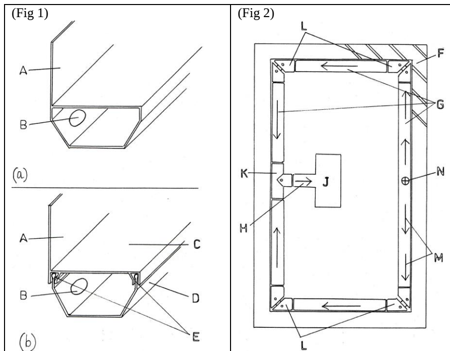
Figures 1 and 2: Sectional and plan drawings of the perimeter floor drain.
