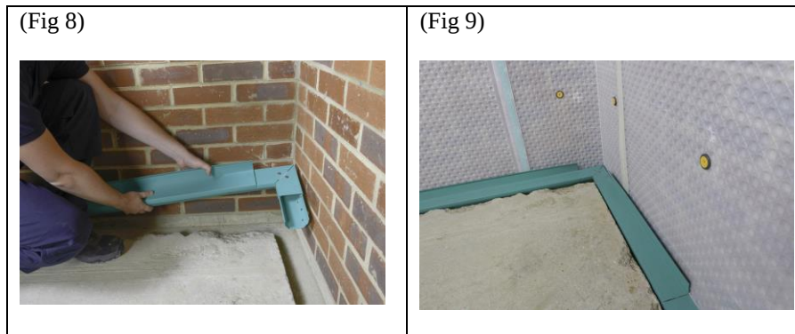
Figures 8 and 9: Photos of the newly designed, easy to fit, perimeter floor drain being installed by a semi-skilled professional in a basement apartment.
