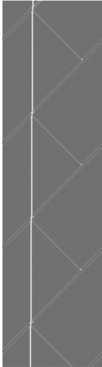
Figure 22. ECA rule 54 evolution implements a simple flip-flop.
