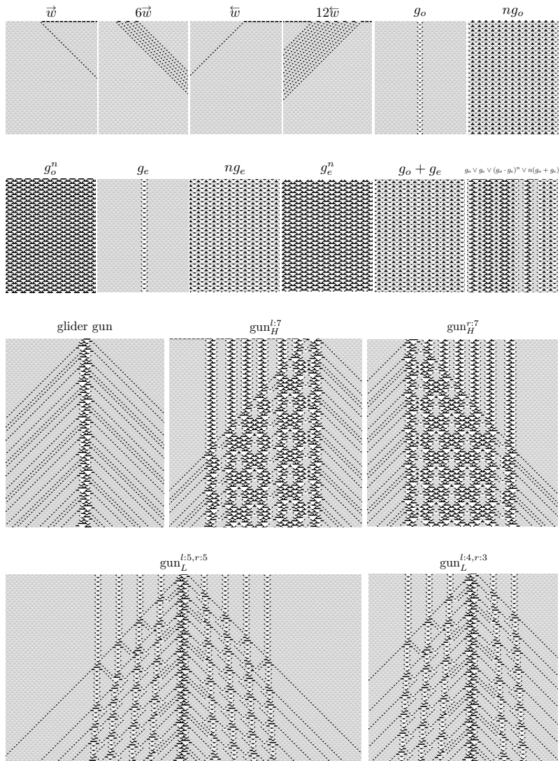
Figure 6. Classification of gliders in rule 54. We illustrate every glider and packages, extensions, and compositions of them.
