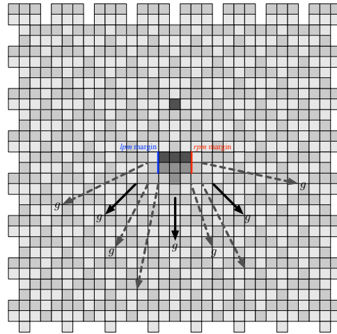
Figure 2. Periodic background in rule 54 is composed with two tiles of the set \mathcal{T}_{R54} : T_1 and T_3^\alpha .
