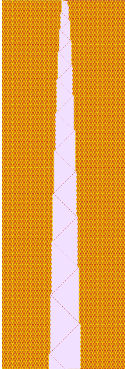
Figure 21. ECA rule 54 evolution deriving a parity function.
