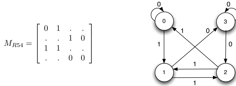
Figure 7. de Bruijn diagram of rule 54.
