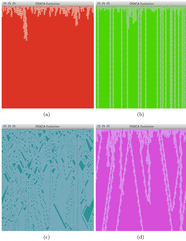
Figure 19. Rule 54 affected with memory functions. (a) ECAM \phi_{R54maj:6} , (b) ECAM \phi_{R54maj:10} , (c) ECAM \phi_{R54maj:3} , (d) ECAM \phi_{R54maj:8} .
