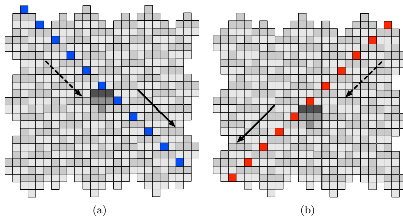
Figure 4. Tiles description for primitive gliders in rule 54.
