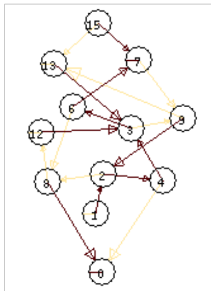
Figure 12. The scalar subset diagram of rule 54.
