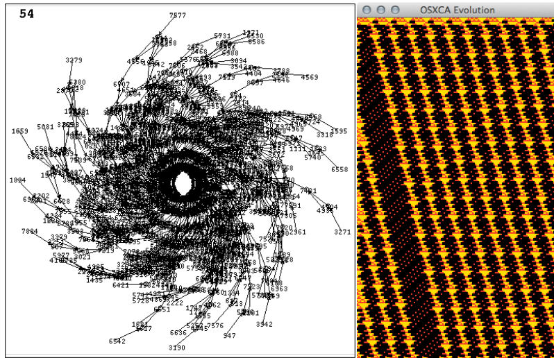
Figure 15. A cycle diagram 13 cells calculating a meta-glider or agar configuration in rule 54.
