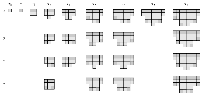
Figure 3. Examples of tiles \mathcal{T}_{R54} derived from space-time configurations in rule 54.
