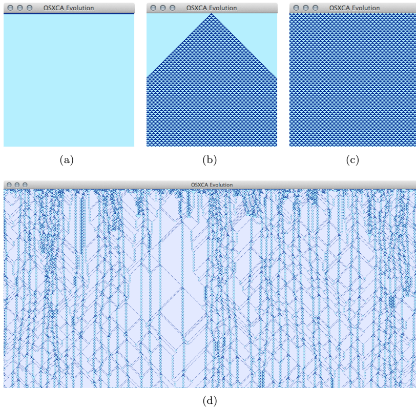
Figure 1. Exemplar scenarios of space-time evolution in rule 54 with 100 cells for 100 generations. (a) A single state of \Sigma dominates the initial condition. (b) A single cell is in state 1; all other cells are in state 0. (c) Periodic background. (d) Random initial condition with an initial density of 50% on 1000 cells for 500 generations (a filter is applied).
