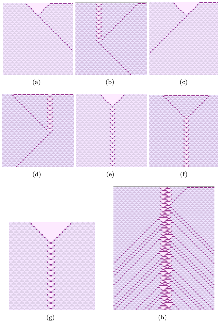
Figure 16. Producing gliders by collisions in rule 54.
