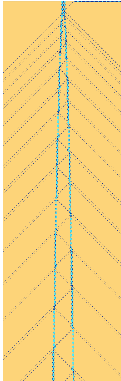
Figure 20. ECA rule 54 evolution deriving a series that yield \mathbb{Z}^n for n > 2 .
