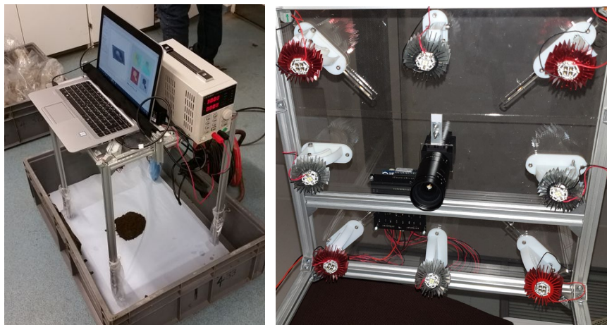
Figure 1. Photograph of the bespoke data capture rig. Left: during an actual sample data capture in laboratory conditions. Right: from below without power supply and laptop. Note that the camera and LEDs are not visible in the left image as they are underneath the computer/power supply.
