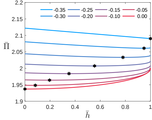
(c) Energy landscape and smooth transition of single equilibrium position for negative CTE.
