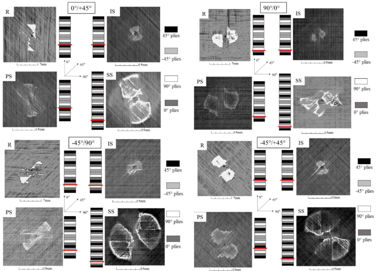
Fig. 13. Delamination at the four respective interfaces 0°/45°, 90°/0°, -45°/90° and 45°/-45° for each S-glass/8552 epoxy configuration. The specific interface where the image was taken is highlighted in red.
