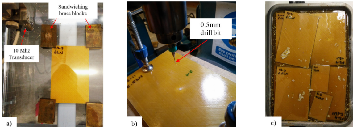
Fig. 4. a) Top view of the C-scan tank; b) Drilling the centre of a tested sample using a 0.5 mm drill bit; c) Dye penetrant bath of drilled samples.
