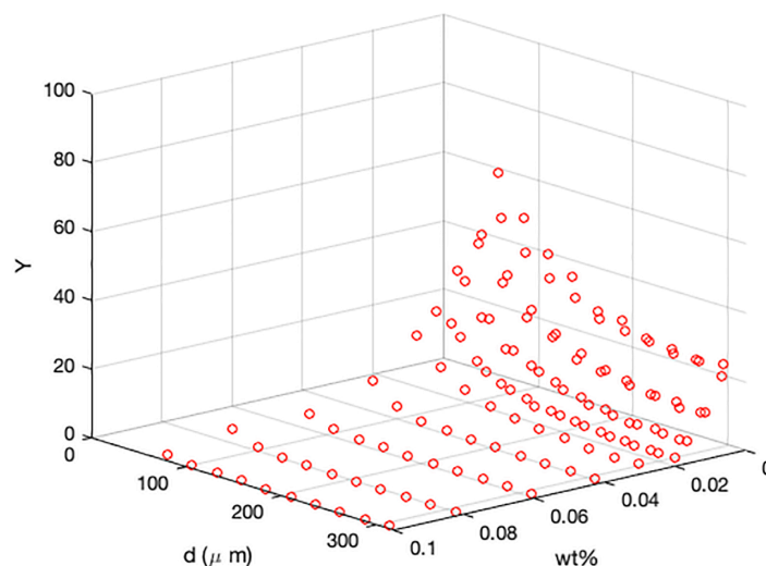
Figure 4 CIE luminance as function of carbon black concentration and optical path length in the dried gelatin layer from (Leech, et al., 2019)
