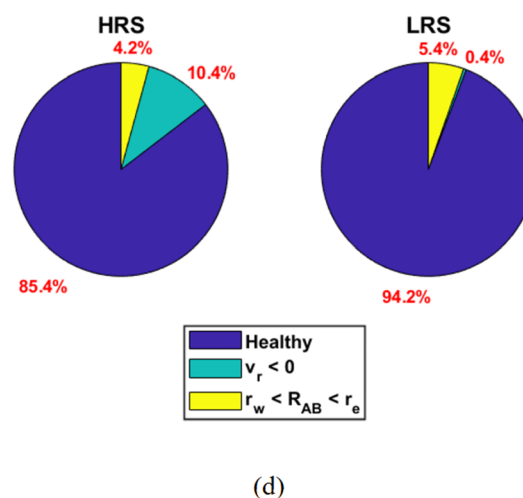
Fig. 7 (a) Flowchart for switching the EMG ferrofluid's resistance between HRS and LRS in pulse mode, (b) endurance test results of 10 million switching cycles between the LRS and HRS using a mean read voltage of 14 mV, (c) yield distribution of the HRS and LRS values for 10 million cycles using a mean read voltage of 14 mV, (d) factors affecting the yield of the HRS and LRS values.
