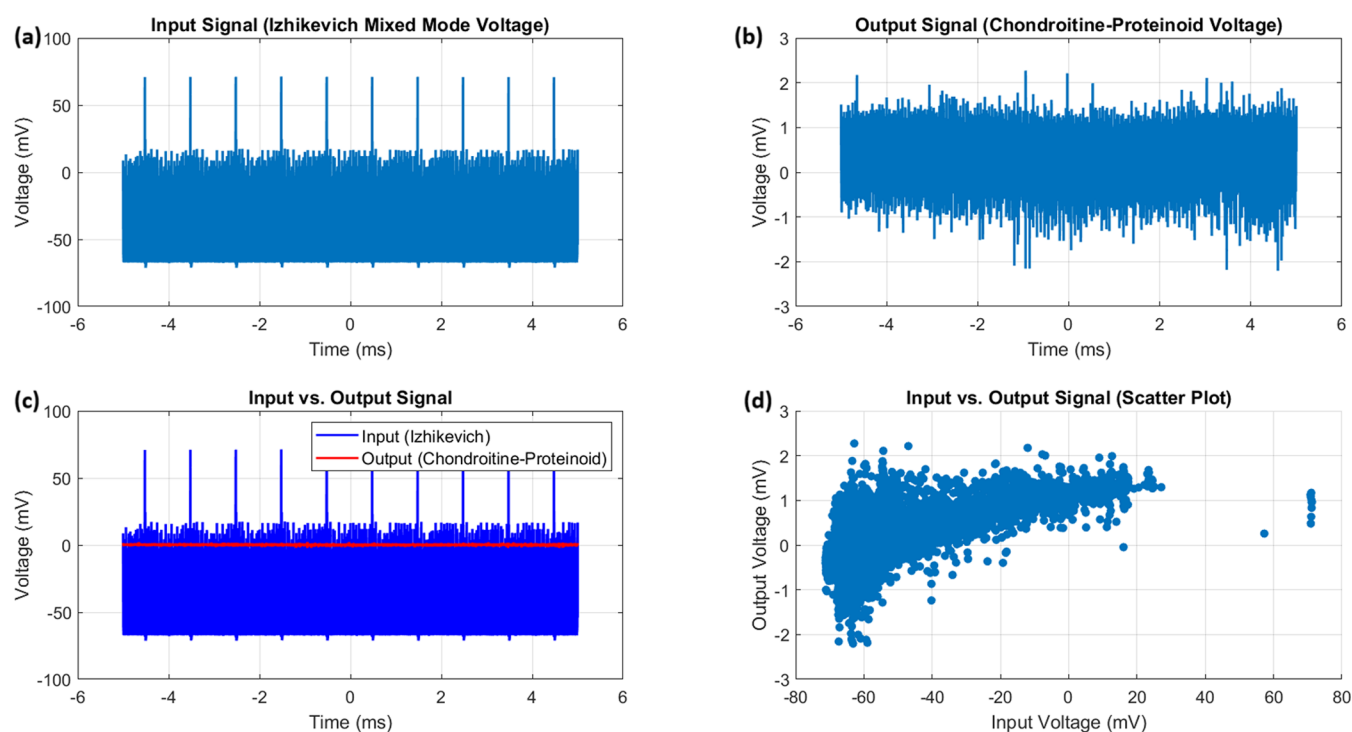
Figure 8. Mixed mode response of the proteinoïd-chondroitine sample to Izhikevich voltage input. (a) The Izhikevich mixed mode voltage input signal exhibits a wide dynamic range and high variability. (b) The chondroitine-proteinoid voltage output signal shows a significantly narrower range and reduced variability compared to the input signal. (c) The input vs output signal plot reveals the temporal relationship between the Izhikevich voltage and the chondroitine-proteinoid voltage, with the output signal displaying a smoother and more stable response. (d) The scatter plot illustrates the strong positive correlation between the input and output voltages, indicating the chondroitine-proteinoid system's ability to capture and preserve the essential features of the input signal while transforming and stabilizing it.
