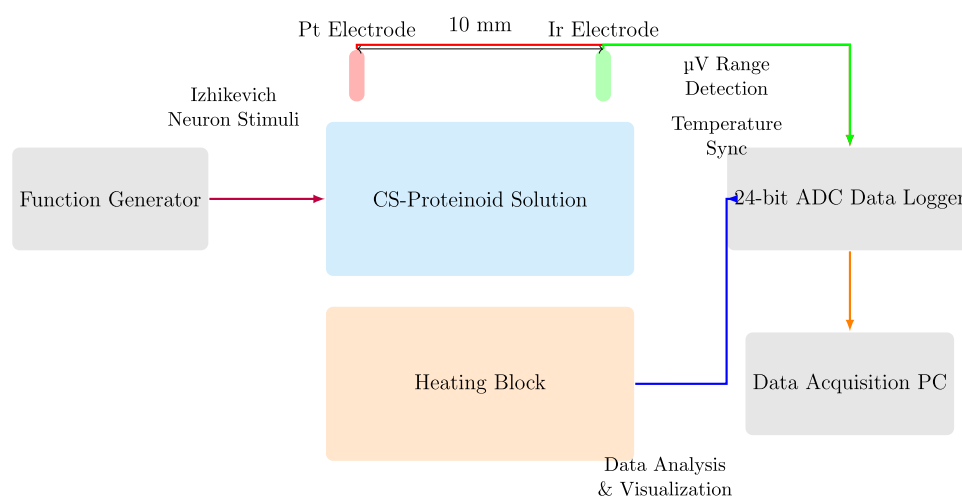
Figure 2. A schematic diagram illustrating the experimental setup used to perform electrochemical characterization of the CS-proteinoid complex. The CS-proteinoid solution with different concentrations of chondroitin sulfate (CS) is contained in the middle container. Two needle electrodes, each plated with platinum (Pt) and iridium (Ir) correspondingly, are placed at a distance of 10 mm from each other in the solution. An ADC data logger with a high level of accuracy, capable of capturing voltage responses in the microvolt ( \mu\text{V} ) range, is used. Additionally, a heating block is employed to regulate and monitor the temperature. A function generator generates stimuli using Izhikevich neuron models. The data acquisition PC gathers, examines, and presents the system's responses. This advanced configuration allows for the identification of small changes in voltage and enables a thorough analysis of voltage responses in the CS-proteinoid system.
