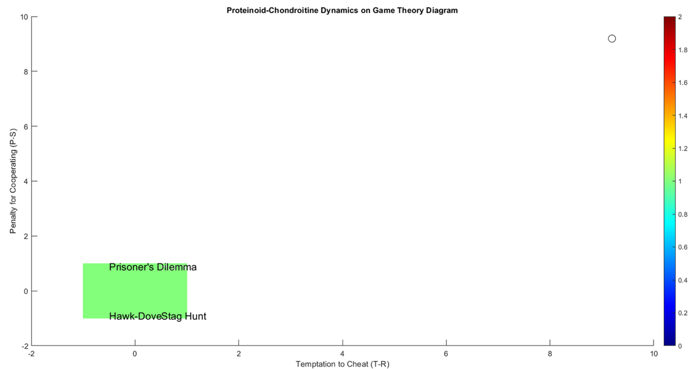
Figure 9. (a) A diagram illustrating the interactions between wild-type (WT) and GASP mutant microspheres in the proteinoid-chondroitine system, mapped onto the temptation to cheat (T-R) and penalty for cooperating (P-S) axes, is presented in the game theory analysis. The diagram is divided into four regimes, each representing different outcomes of cooperation and defection: Harmony, Hawk-Dove, Stag Hunt, and Prisoner's Dilemma. The colormap represents the equilibrium state of the population, showing the proportion of cooperators. Warmer colors, such as red, indicate a higher fraction of cooperators, while cooler colors, like blue, suggest a lower fraction. The position on the diagram that corresponds to the payoff matrix of the proteinoid-chondroitine system (which is not displayed) would determine the game theoretical regime and the anticipated long-term result of cooperation or defection in the system. (b) Proteinoid-chondroitine dynamics mapped onto the game theory diagram. The white point represents the current scenario based on the calculated temptation to cheat (T-R) and penalty for cooperating (P-S) values. The dynamics fall within the Prisoner's Dilemma regime, suggesting that defection is likely to be the long-term outcome in the system.
