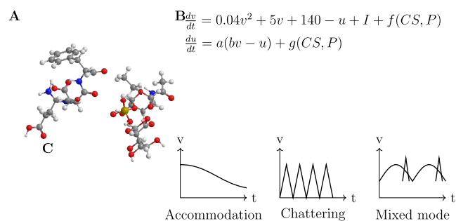
Figure 1. Key concepts in CS-Proteinoid modulation of neuronal dynamics. (A) Structure and interaction of chondroitin sulfate (CS) and proteinoid. (B) Modified Izhikevich model equations incorporating CS-Proteinoid effects. (C) Examples of firing patterns modulated by CS-Proteinoid mixtures: accommodation, chattering, and mixed mode oscillations.
