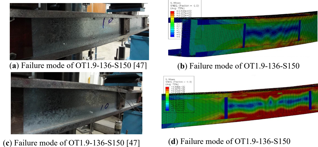
Figure 17. Comparison of experimental [47] and FE failure modes for cold-formed steel built-up open section OT1.9-136-S150 and OT1.9-136-S300.
