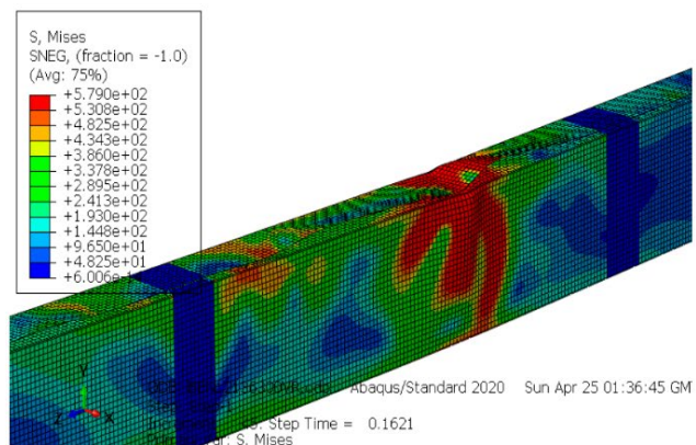
(f) Failure mode of CT1.2-136-S600
