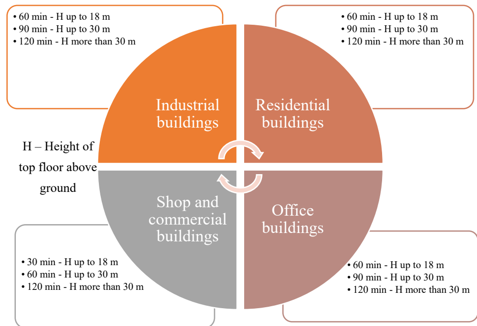
Figure 10. Minimum fire resistance period [59].
