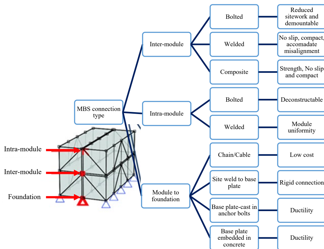
Figure 8. Modular connection types [53].
