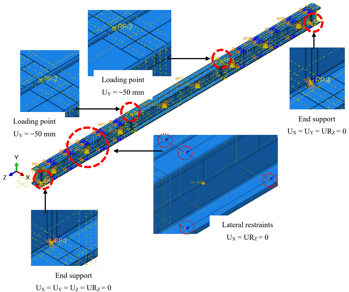
Figure 16. Boundary conditions at loading, supporting and strap points.
